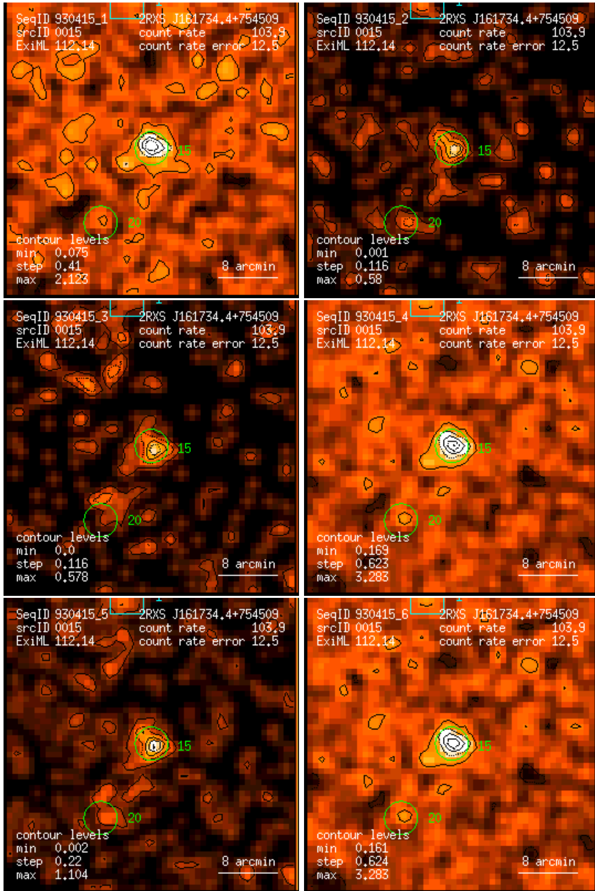
Figure 15: RASS 930415: detection 0015: band rate images, Gaussian filter: (1) PSPC channels 11 – 41, (2) 52 – 90, (3) 91 – 201, (4) 11 – 235, (5) 52 – 201, (6) 11 – 201. Broad band rates in counts/ks. Band rate contour levels in counts/ks/arcmin 2 .
