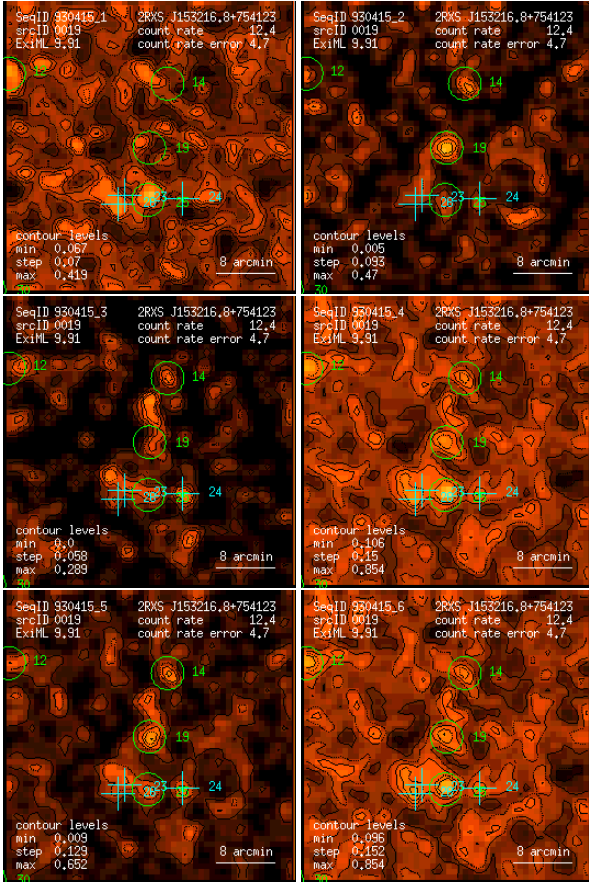
Figure 19: RASS 930415: detection 0019: band rate images, Gaussian filter: (1) PSPC channels 11 – 41, (2) 52 – 90, (3) 91 – 201, (4) 11 – 235, (5) 52 – 201, (6) 11 – 201. Broad band rates in counts/ks. Band rate contour levels in counts/ks/arcmin 2 .
