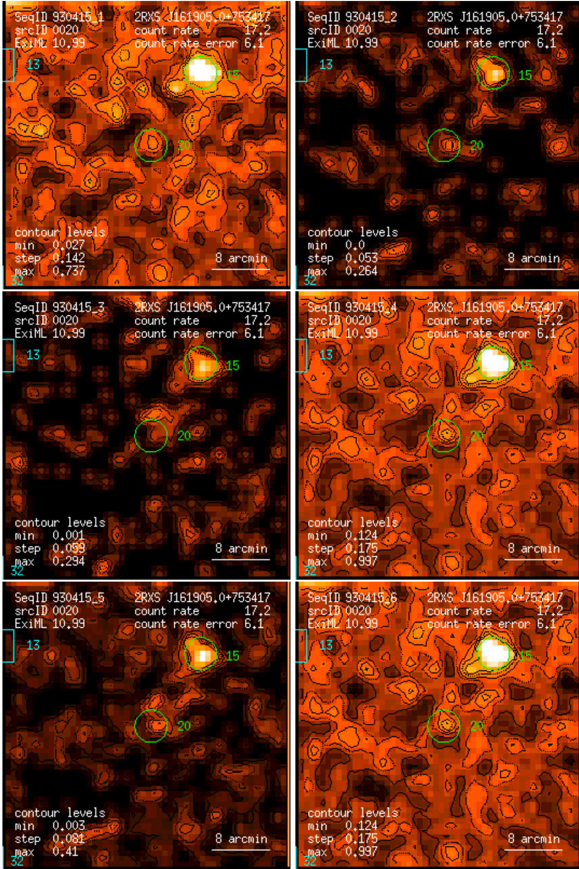
Figure 20: RASS 930415: detection 0020: band rate images, Gaussian filter: (1) PSPC channels 11 – 41, (2) 52 – 90, (3) 91 – 201, (4) 11 – 235, (5) 52 – 201, (6) 11 – 201. Broad band rates in counts/ks. Band rate contour levels in counts/ks/arcmin 2 .
