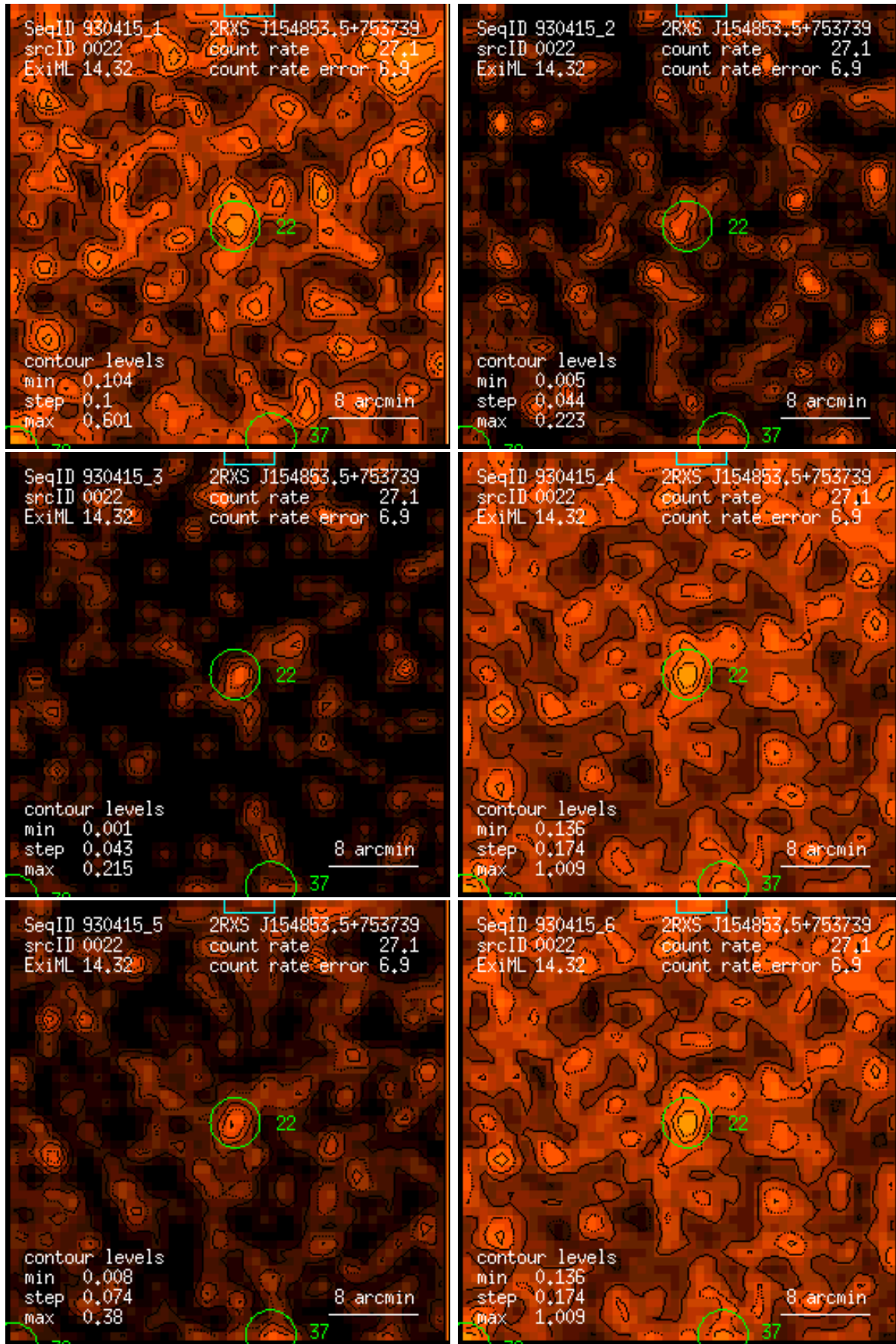
Figure 22: RASS 930415: detection 0022: band rate images, Gaussian filter: (1) PSPC channels 11 – 41, (2) 52 – 90, (3) 91 – 201, (4) 11 – 235, (5) 52 – 201, (6) 11 – 201. Broad band rates in counts/ks. Band rate contour levels in counts/ks/arcmin 2 .
