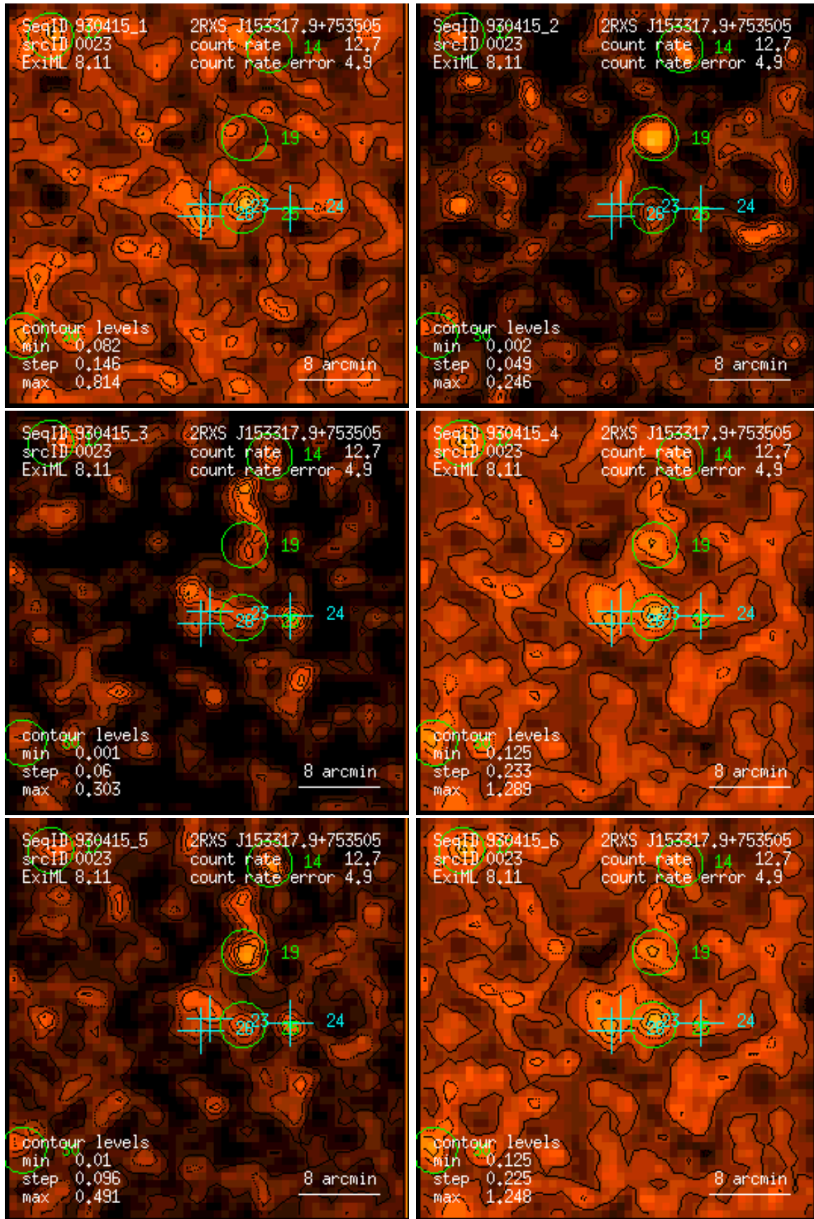
Figure 23: RASS 930415: detection 0023: band rate images, Gaussian filter: (1) PSPC channels 11 – 41, (2) 52 – 90, (3) 91 – 201, (4) 11 – 235, (5) 52 – 201, (6) 11 – 201. Broad band rates in counts/ks. Band rate contour levels in counts/ks/arcmin 2 .
