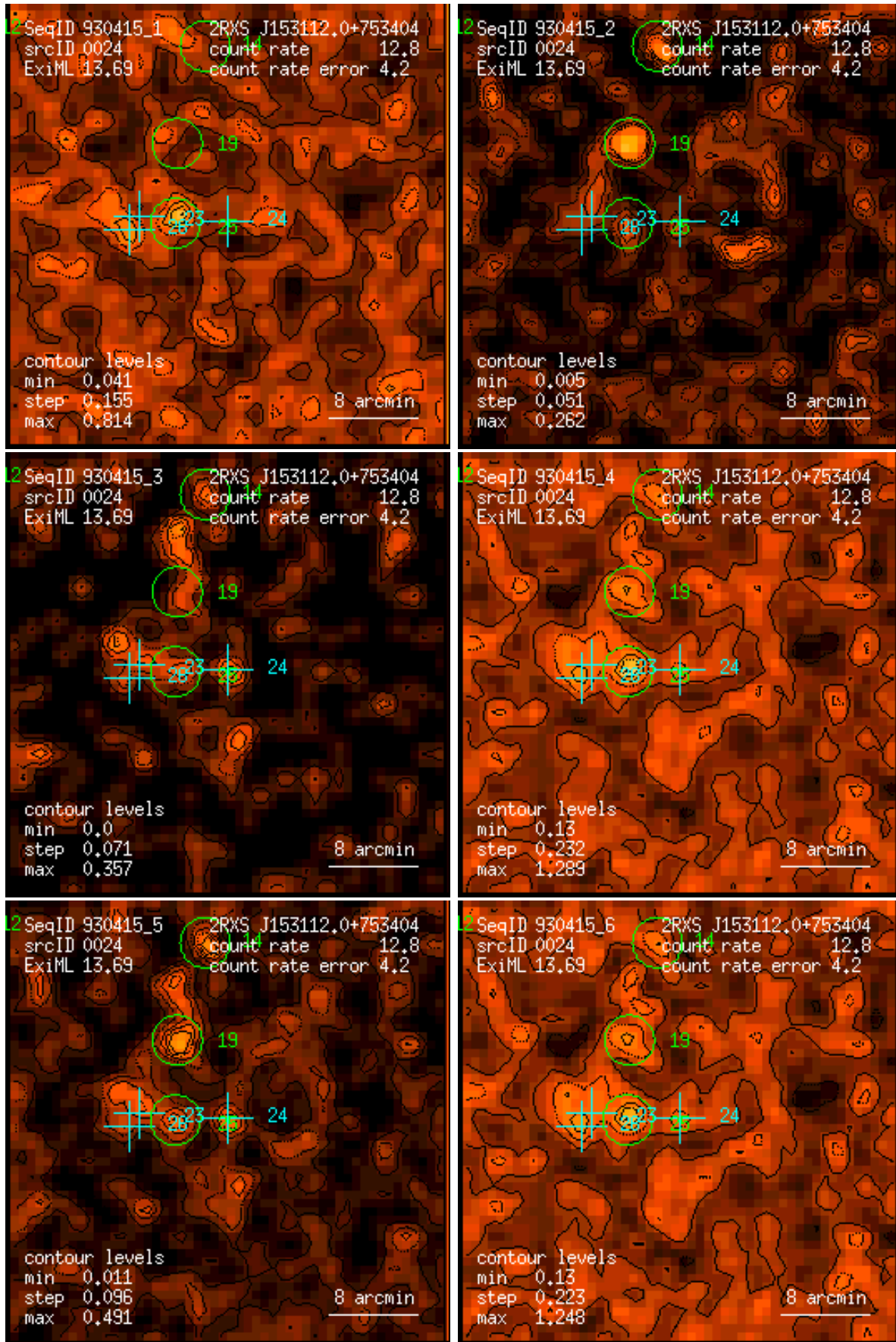
Figure 24: RASS 930415: detection 0024: band rate images, Gaussian filter: (1) PSPC channels 11 – 41, (2) 52 – 90, (3) 91 – 201, (4) 11 – 235, (5) 52 – 201, (6) 11 – 201. Broad band rates in counts/ks. Band rate contour levels in counts/ks/arcmin 2 .
