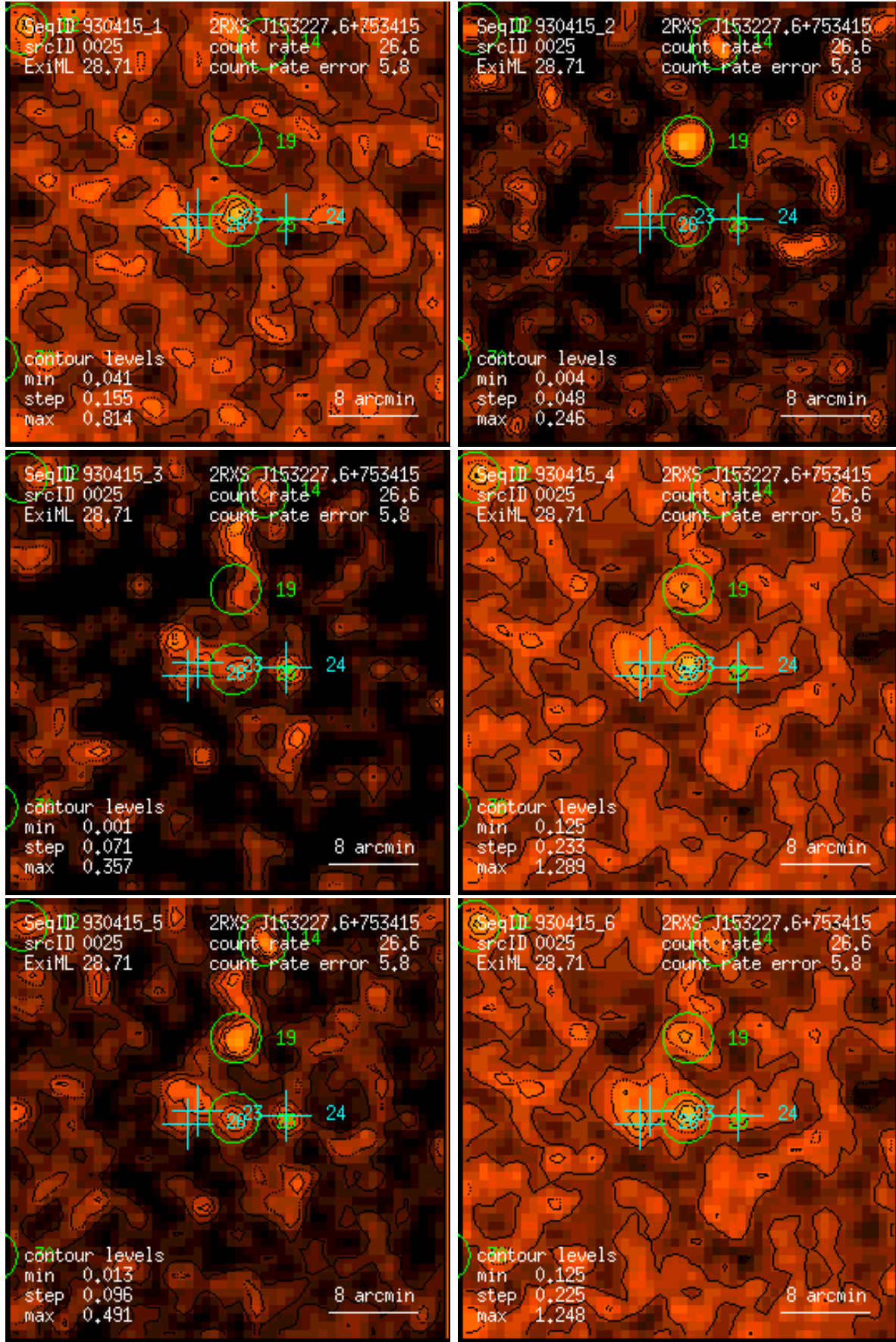
Figure 25: RASS 930415: detection 0025: band rate images, Gaussian filter: (1) PSPC channels 11 – 41, (2) 52 – 90, (3) 91 – 201, (4) 11 – 235, (5) 52 – 201, (6) 11 – 201. Broad band rates in counts/ks. Band rate contour levels in counts/ks/arcmin 2 .
