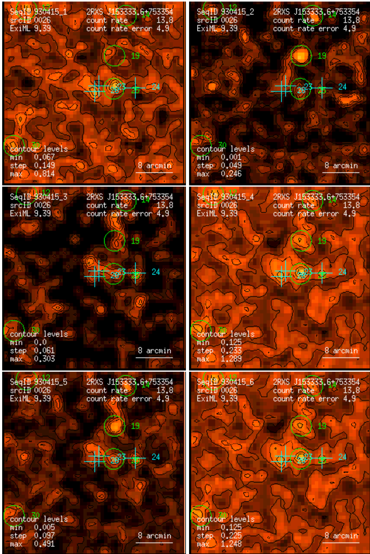
Figure 26: RASS 930415: detection 0026: band rate images, Gaussian filter: (1) PSPC channels 11 – 41, (2) 52 – 90, (3) 91 – 201, (4) 11 – 235, (5) 52 – 201, (6) 11 – 201. Broad band rates in counts/ks. Band rate contour levels in counts/ks/arcmin 2 .
