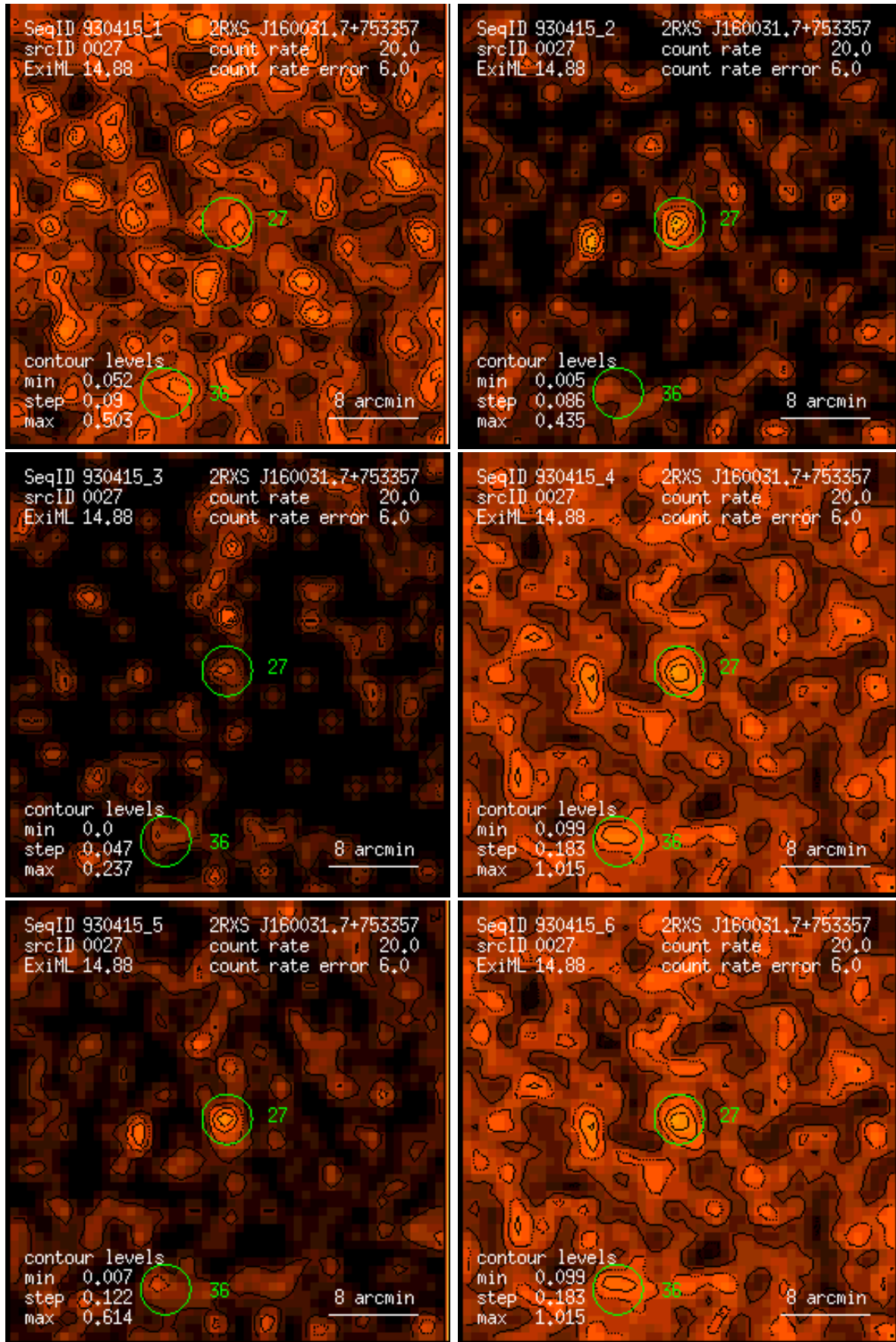
Figure 27: RASS 930415: detection 0027: band rate images, Gaussian filter: (1) PSPC channels 11 – 41, (2) 52 – 90, (3) 91 – 201, (4) 11 – 235, (5) 52 – 201, (6) 11 – 201. Broad band rates in counts/ks. Band rate contour levels in counts/ks/arcmin 2 .
