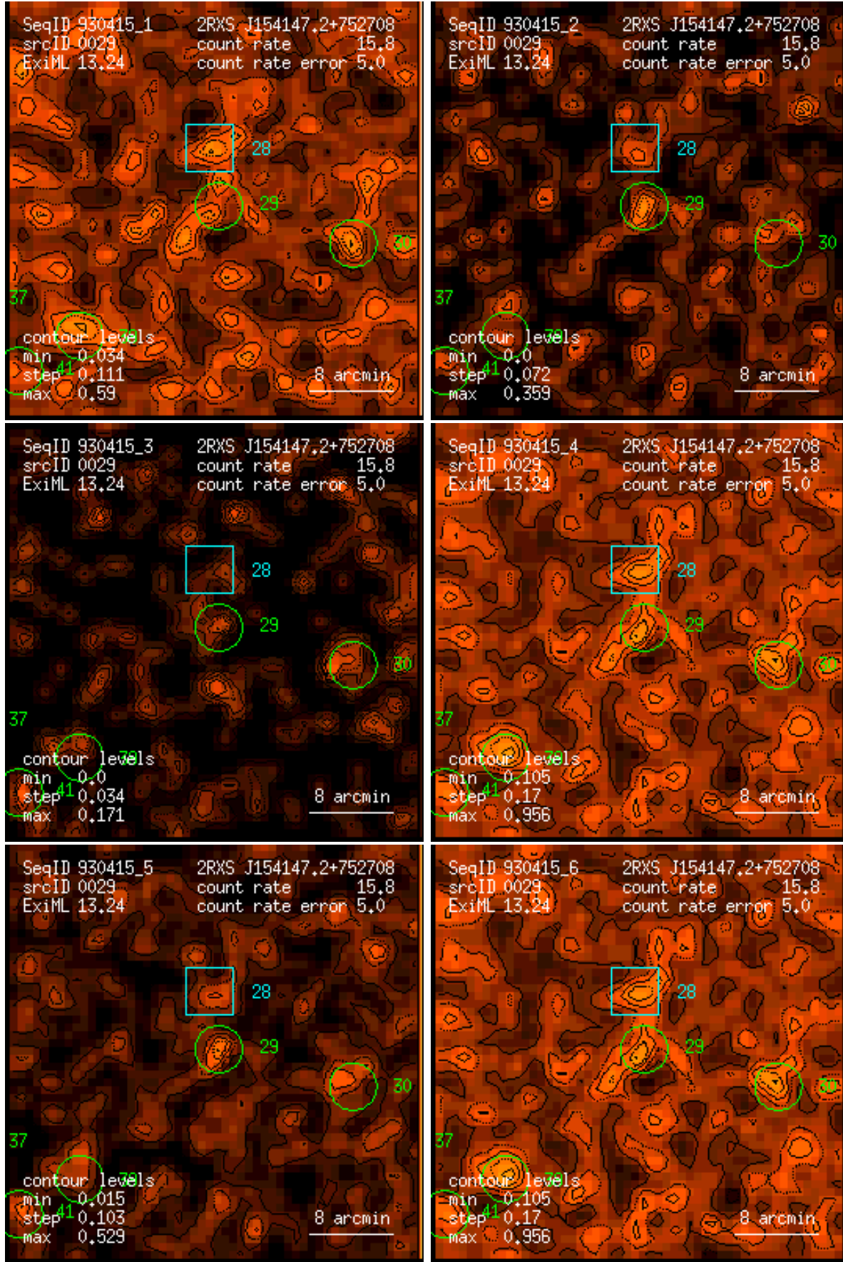
Figure 29: RASS 930415: detection 0029: band rate images, Gaussian filter: (1) PSPC channels 11 – 41, (2) 52 – 90, (3) 91 – 201, (4) 11 – 235, (5) 52 – 201, (6) 11 – 201. Broad band rates in counts/ks. Band rate contour levels in counts/ks/arcmin 2 .
