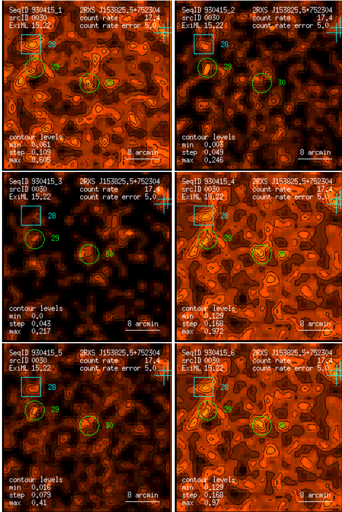
Figure 30: RASS 930415: detection 0030: band rate images, Gaussian filter: (1) PSPC channels 11 – 41, (2) 52 – 90, (3) 91 – 201, (4) 11 – 235, (5) 52 – 201, (6) 11 – 201. Broad band rates in counts/ks. Band rate contour levels in counts/ks/arcmin 2 .
