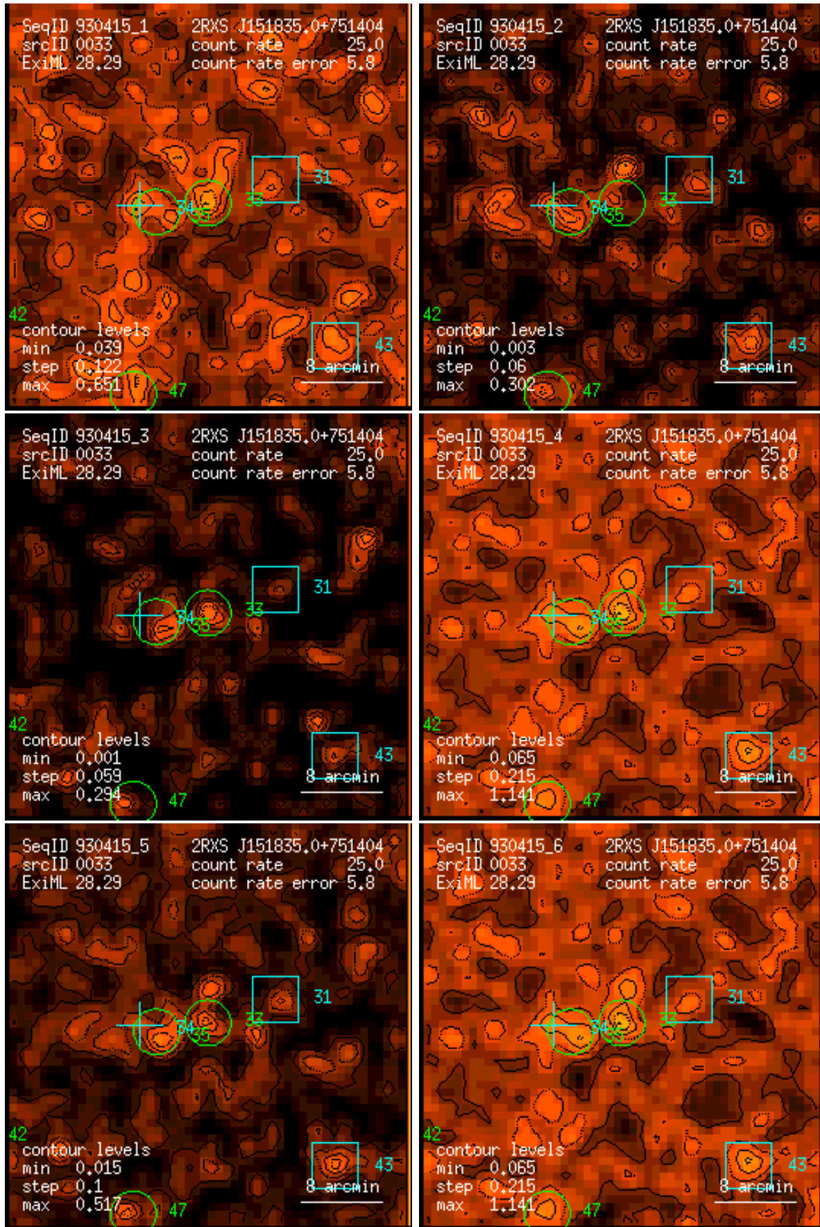
Figure 33: RASS 930415: detection 0033: band rate images, Gaussian filter: (1) PSPC channels 11 – 41, (2) 52 – 90, (3) 91 – 201, (4) 11 – 235, (5) 52 – 201, (6) 11 – 201. Broad band rates in counts/ks. Band rate contour levels in counts/ks/arcmin 2 .
