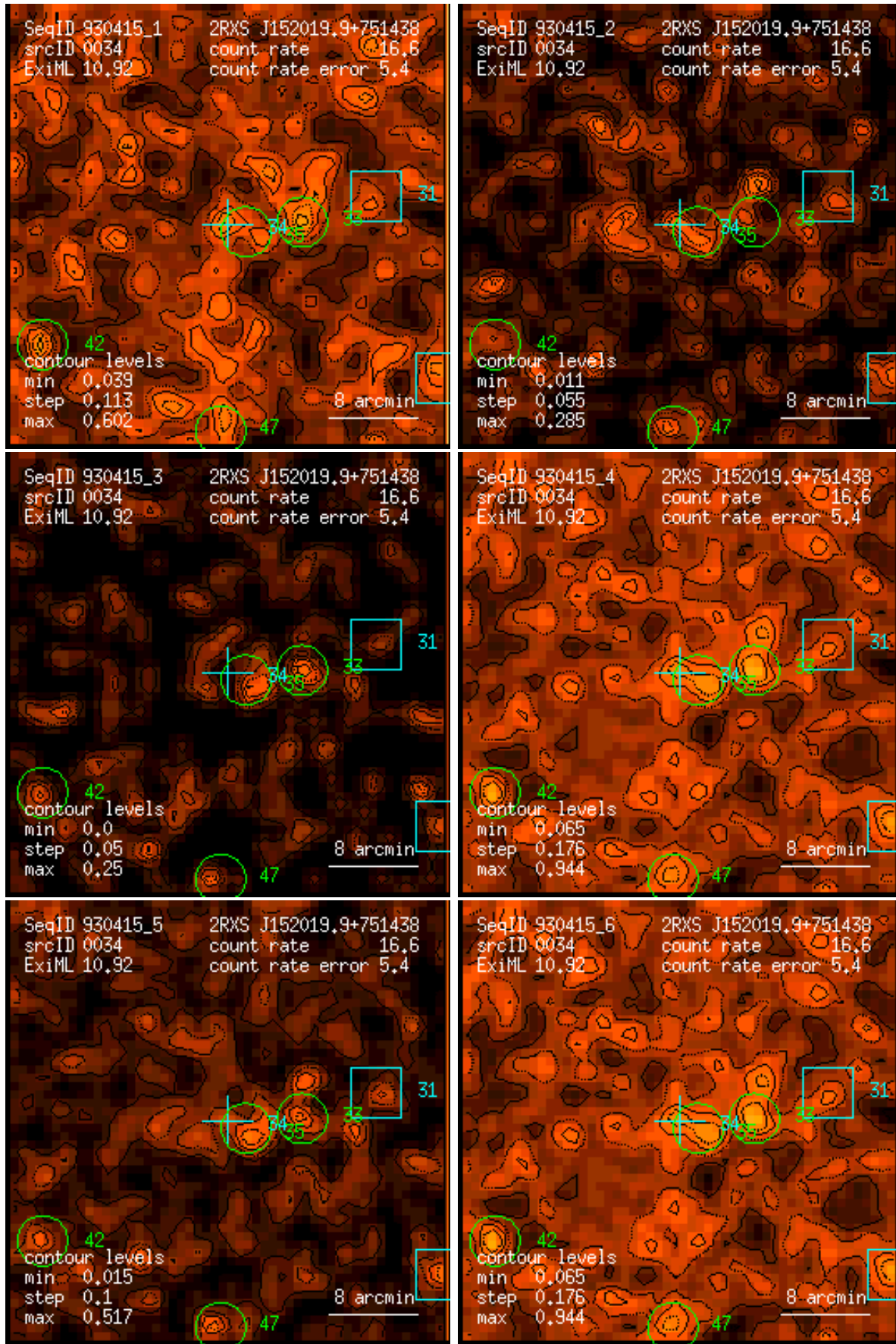
Figure 34: RASS 930415: detection 0034: band rate images, Gaussian filter: (1) PSPC channels 11 – 41, (2) 52 – 90, (3) 91 – 201, (4) 11 – 235, (5) 52 – 201, (6) 11 – 201. Broad band rates in counts/ks. Band rate contour levels in counts/ks/arcmin 2 .
