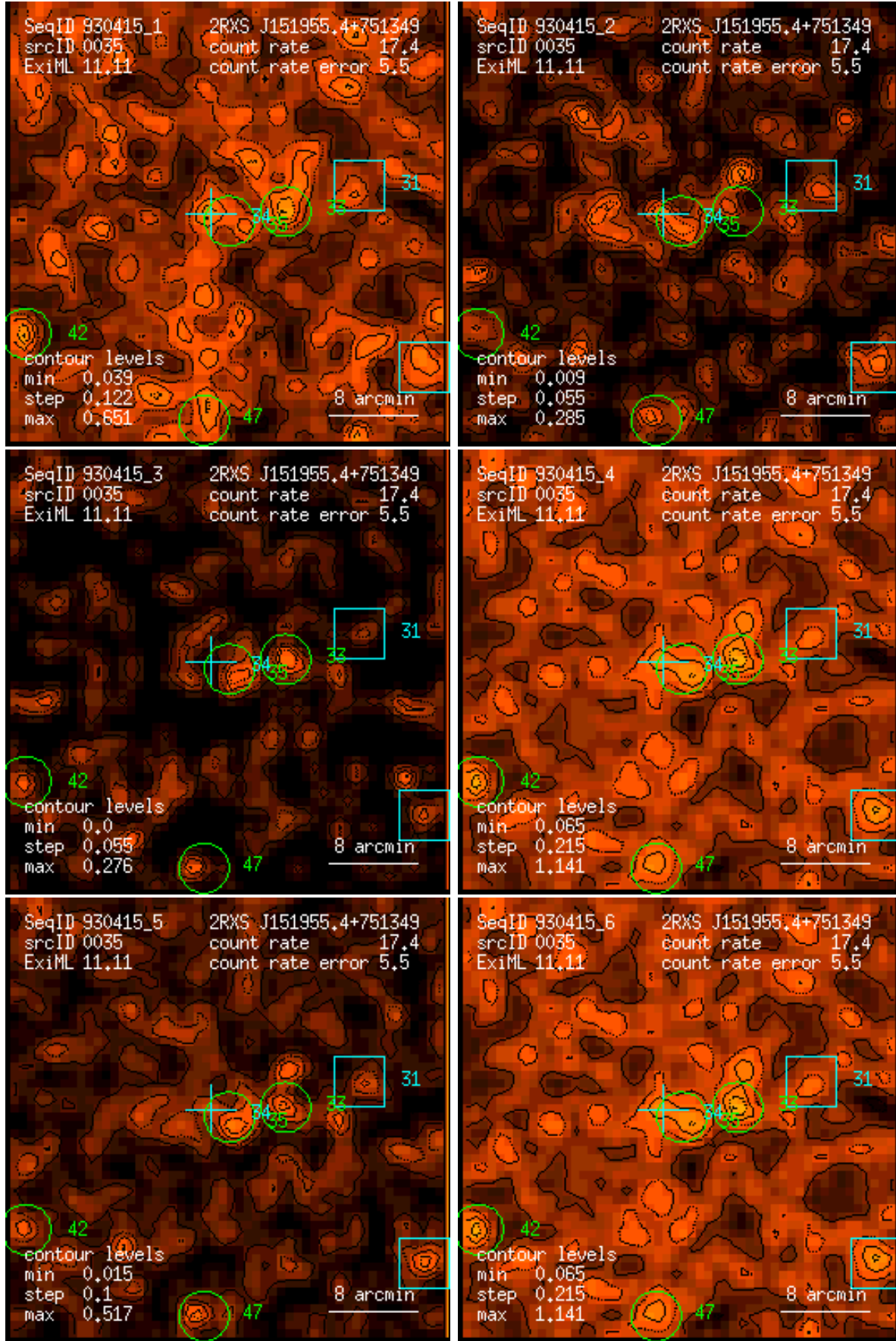
Figure 35: RASS 930415: detection 0035: band rate images, Gaussian filter: (1) PSPC channels 11 – 41, (2) 52 – 90, (3) 91 – 201, (4) 11 – 235, (5) 52 – 201, (6) 11 – 201. Broad band rates in counts/ks. Band rate contour levels in counts/ks/arcmin 2 .
