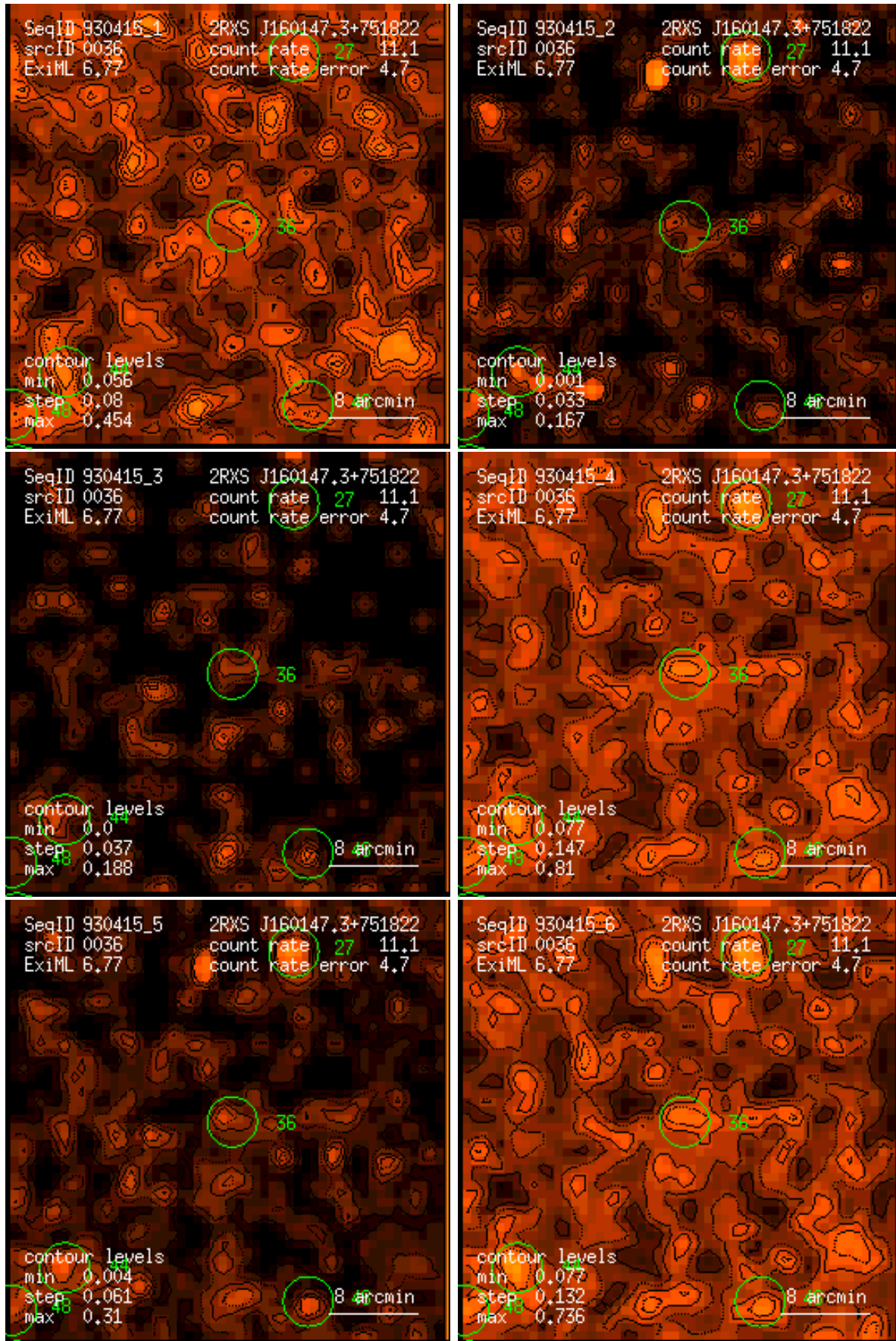
Figure 36: RASS 930415: detection 0036: band rate images, Gaussian filter: (1) PSPC channels 11 – 41, (2) 52 – 90, (3) 91 – 201, (4) 11 – 235, (5) 52 – 201, (6) 11 – 201. Broad band rates in counts/ks. Band rate contour levels in counts/ks/arcmin 2 .
