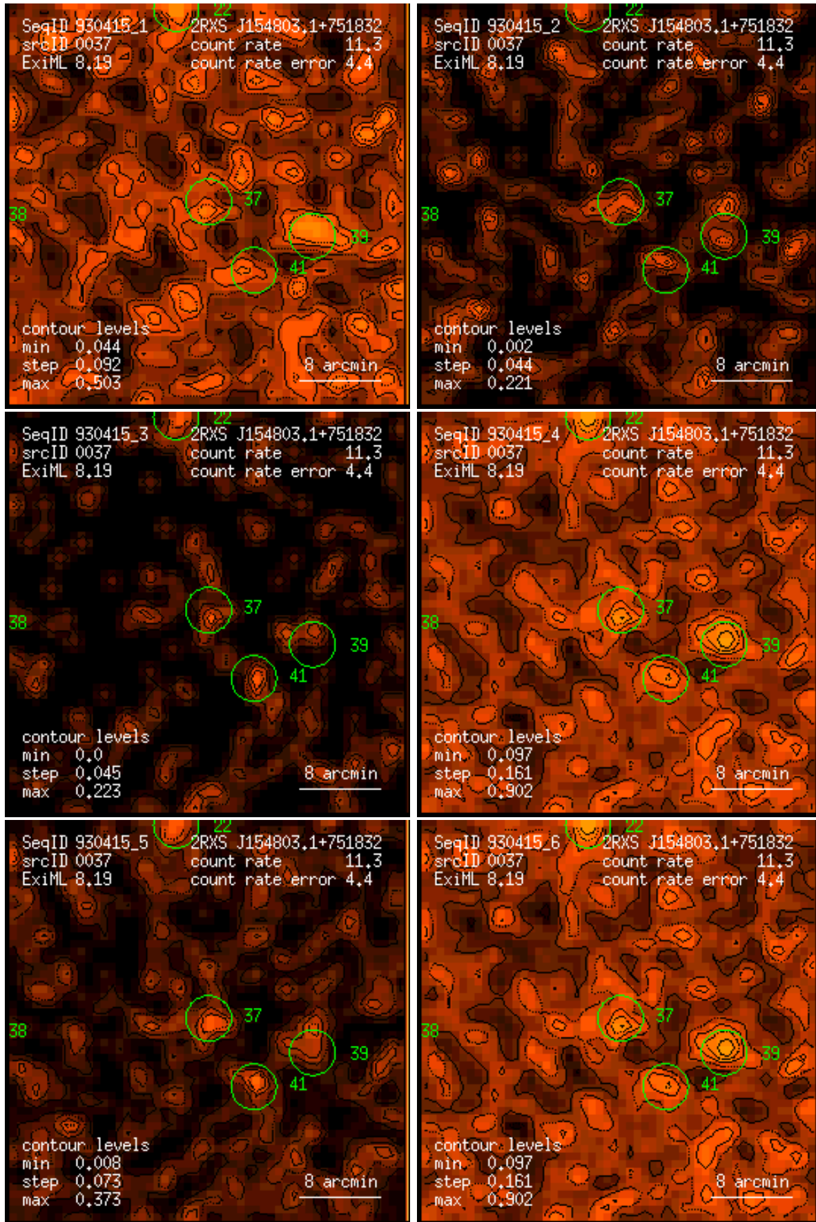
Figure 37: RASS 930415: detection 0037: band rate images, Gaussian filter: (1) PSPC channels 11 – 41, (2) 52 – 90, (3) 91 – 201, (4) 11 – 235, (5) 52 – 201, (6) 11 – 201. Broad band rates in counts/ks. Band rate contour levels in counts/ks/arcmin 2 .
