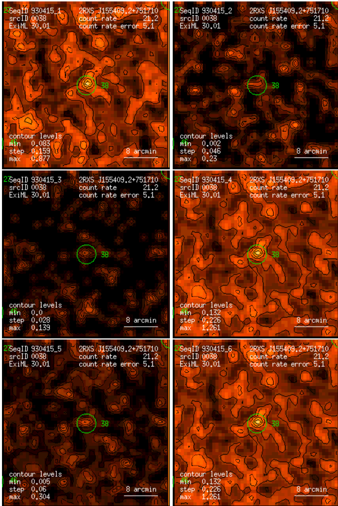
Figure 38: RASS 930415: detection 0038: band rate images, Gaussian filter: (1) PSPC channels 11 – 41, (2) 52 – 90, (3) 91 – 201, (4) 11 – 235, (5) 52 – 201, (6) 11 – 201. Broad band rates in counts/ks. Band rate contour levels in counts/ks/arcmin 2 .
