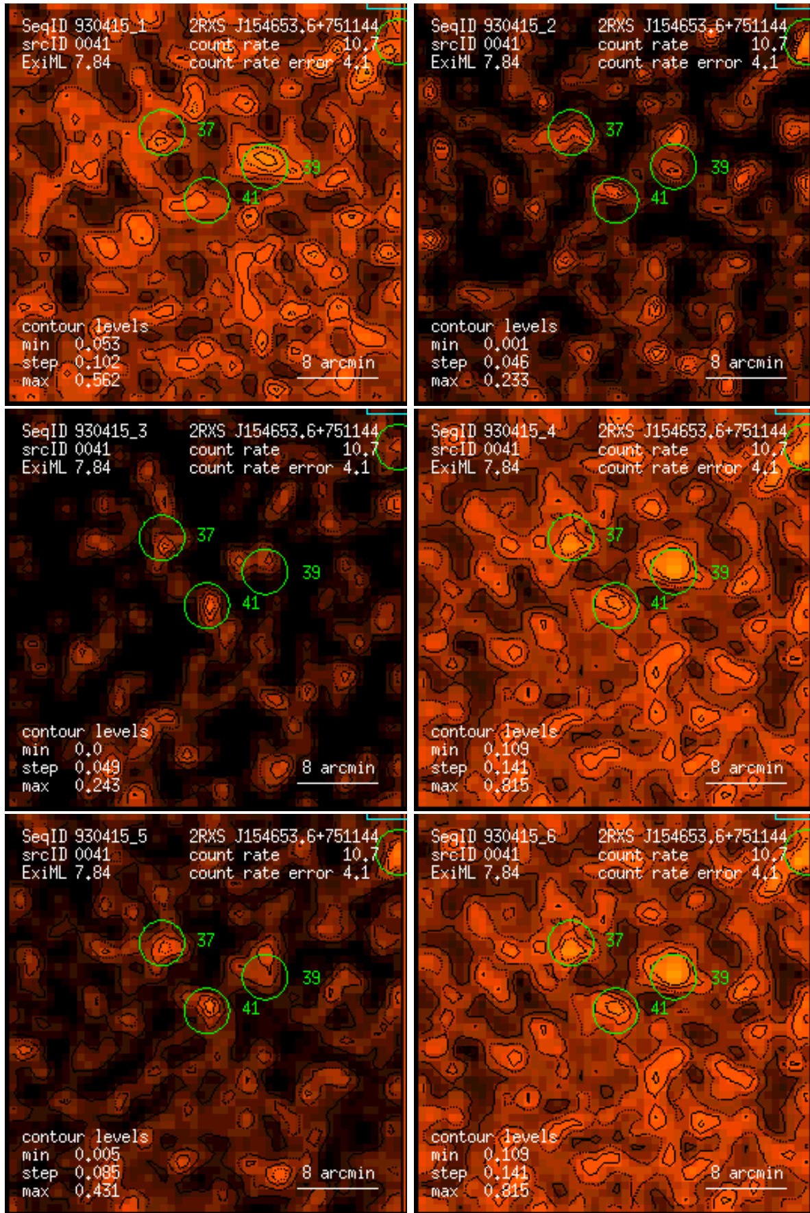
Figure 41: RASS 930415: detection 0041: band rate images, Gaussian filter: (1) PSPC channels 11 – 41, (2) 52 – 90, (3) 91 – 201, (4) 11 – 235, (5) 52 – 201, (6) 11 – 201. Broad band rates in counts/ks. Band rate contour levels in counts/ks/arcmin 2 .
