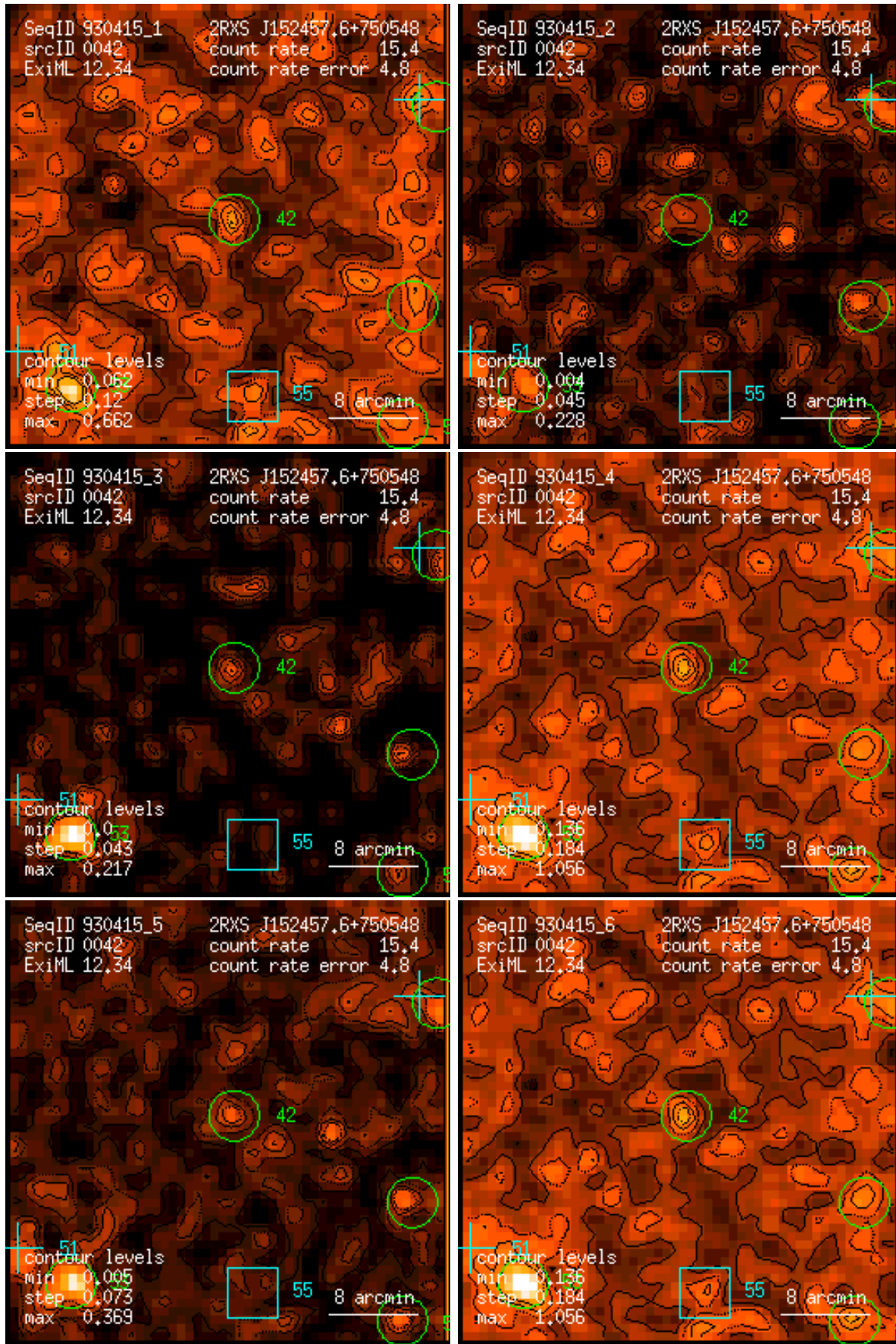
Figure 42: RASS 930415: detection 0042: band rate images, Gaussian filter: (1) PSPC channels 11 – 41, (2) 52 – 90, (3) 91 – 201, (4) 11 – 235, (5) 52 – 201, (6) 11 – 201. Broad band rates in counts/ks. Band rate contour levels in counts/ks/arcmin 2 .
