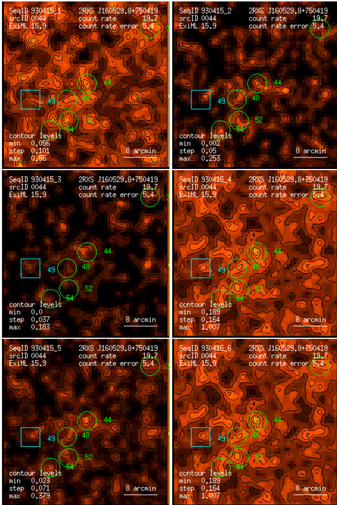
Figure 44: RASS 930415: detection 0044: band rate images, Gaussian filter: (1) PSPC channels 11 – 41, (2) 52 – 90, (3) 91 – 201, (4) 11 – 235, (5) 52 – 201, (6) 11 – 201. Broad band rates in counts/ks. Band rate contour levels in counts/ks/arcmin 2 .
