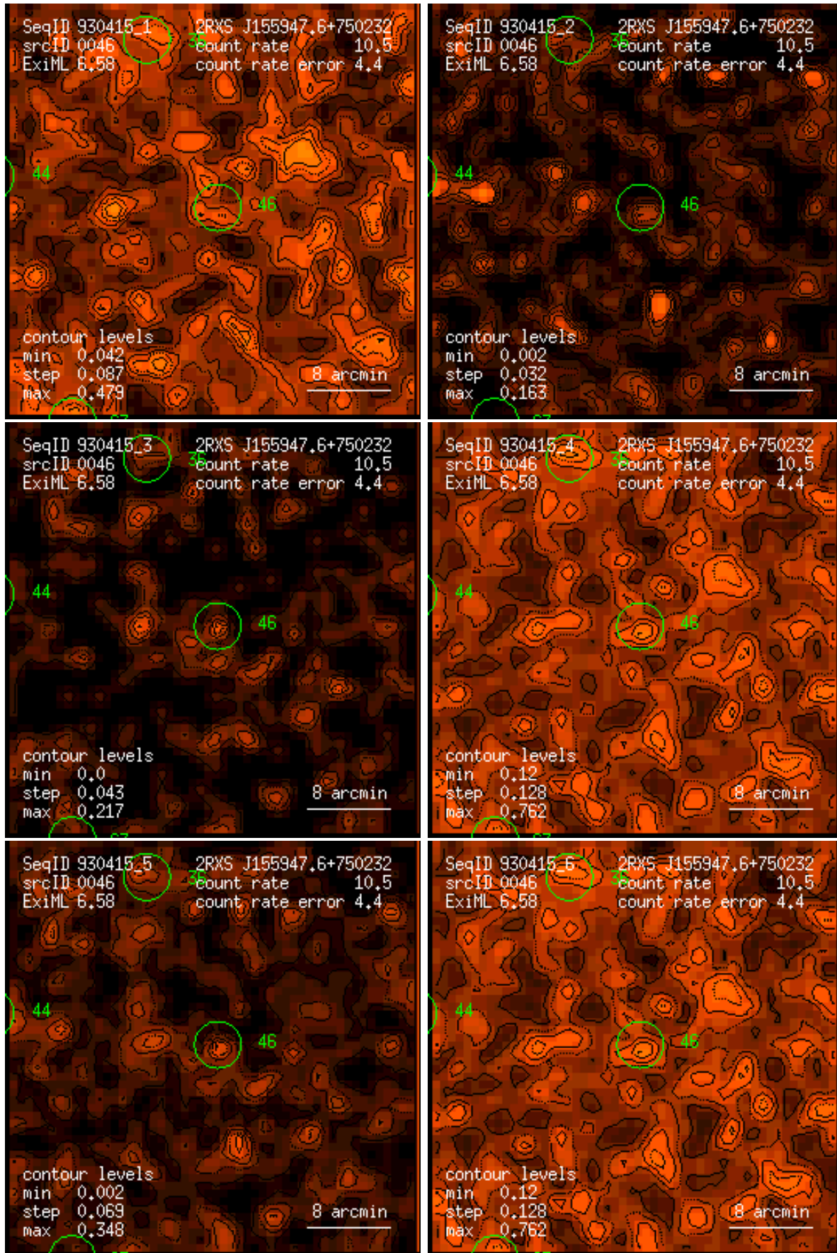
Figure 46: RASS 930415: detection 0046: band rate images, Gaussian filter: (1) PSPC channels 11 – 41, (2) 52 – 90, (3) 91 – 201, (4) 11 – 235, (5) 52 – 201, (6) 11 – 201. Broad band rates in counts/ks. Band rate contour levels in counts/ks/arcmin 2 .
