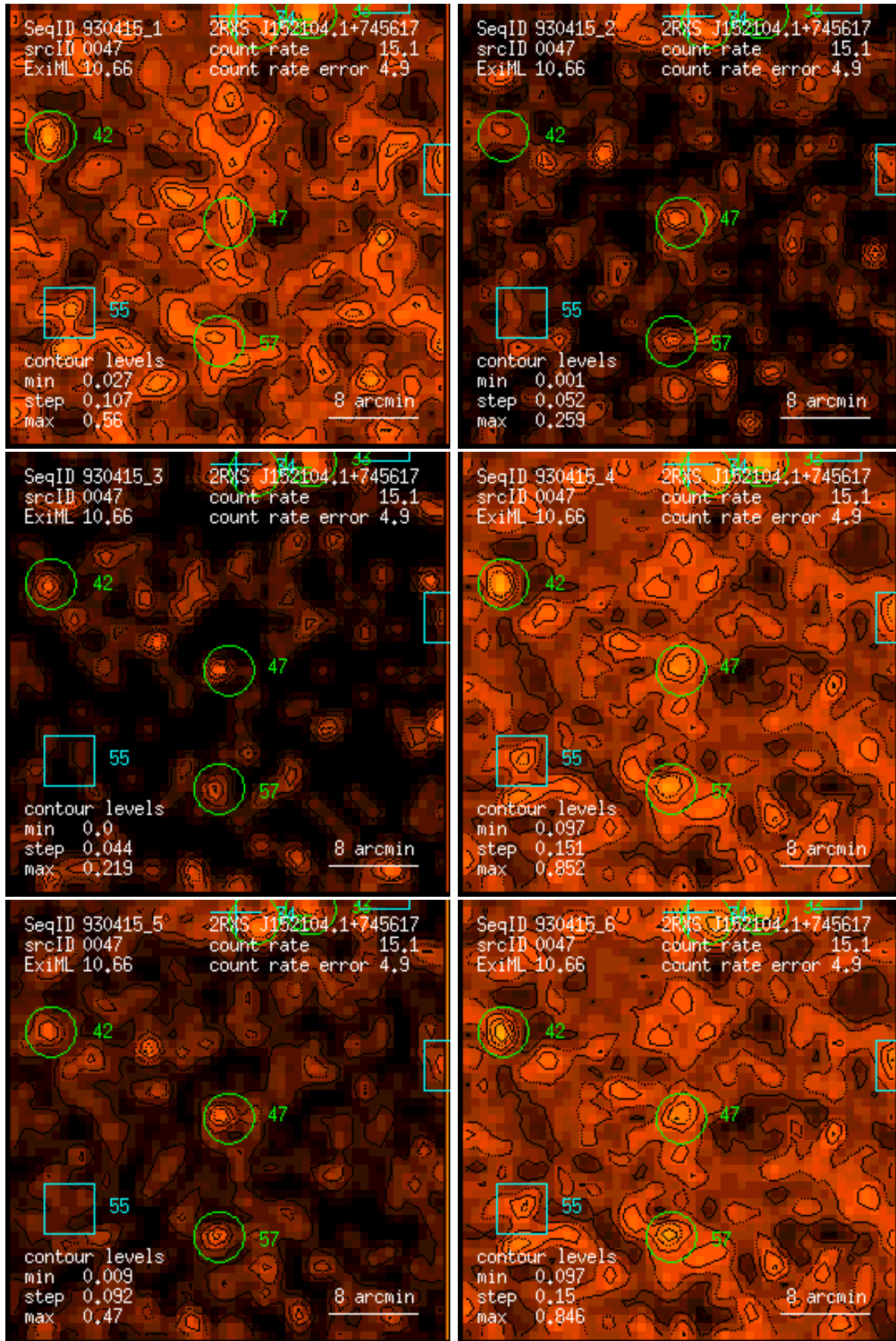
Figure 47: RASS 930415: detection 0047: band rate images, Gaussian filter: (1) PSPC channels 11 – 41, (2) 52 – 90, (3) 91 – 201, (4) 11 – 235, (5) 52 – 201, (6) 11 – 201. Broad band rates in counts/ks. Band rate contour levels in counts/ks/arcmin 2 .
