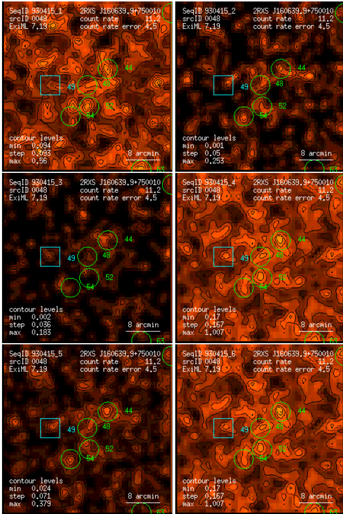
Figure 48: RASS 930415: detection 0048: band rate images, Gaussian filter: (1) PSPC channels 11 – 41, (2) 52 – 90, (3) 91 – 201, (4) 11 – 235, (5) 52 – 201, (6) 11 – 201. Broad band rates in counts/ks. Band rate contour levels in counts/ks/arcmin 2 .
