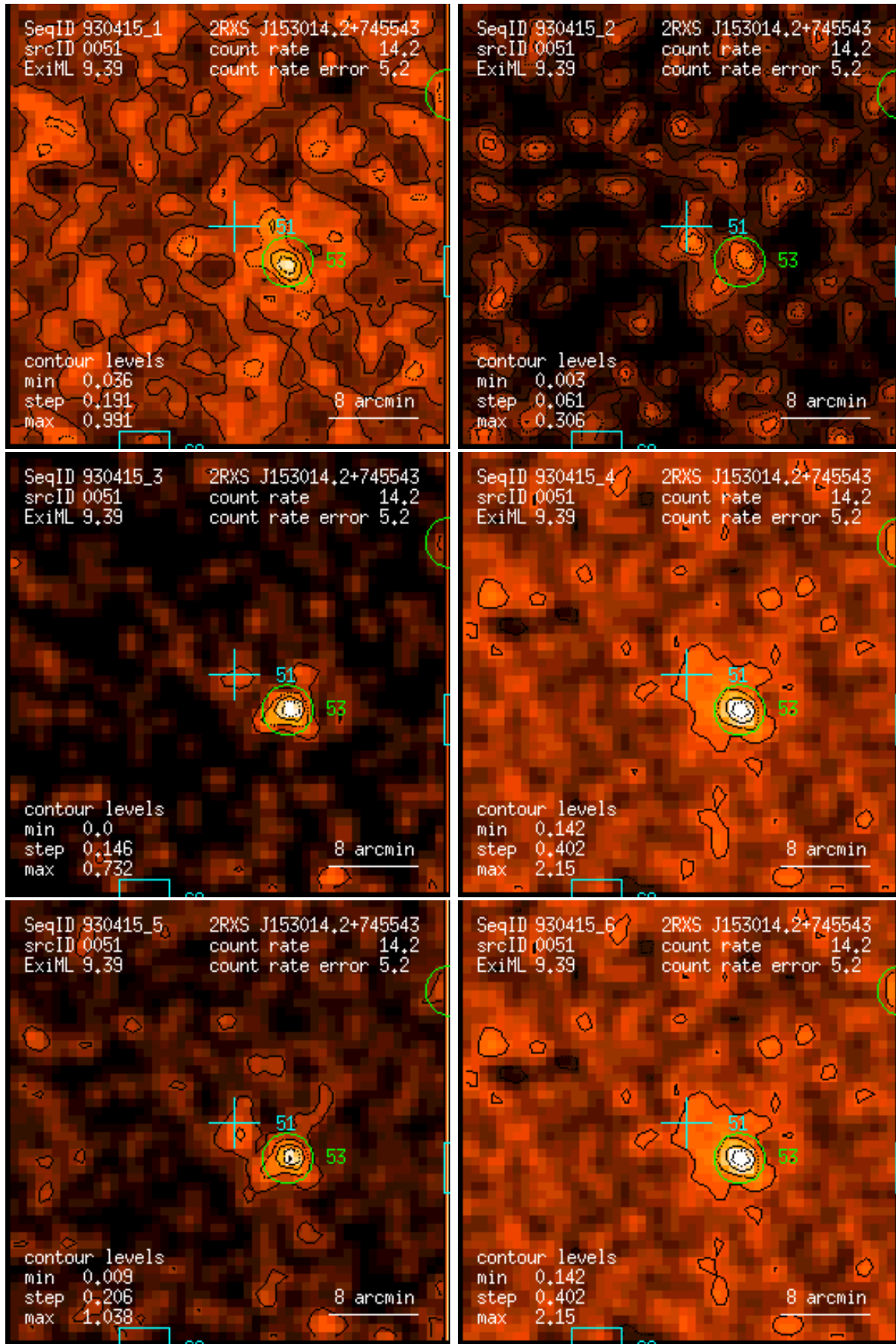
Figure 51: RASS 930415: detection 0051: band rate images, Gaussian filter: (1) PSPC channels 11 – 41, (2) 52 – 90, (3) 91 – 201, (4) 11 – 235, (5) 52 – 201, (6) 11 – 201. Broad band rates in counts/ks. Band rate contour levels in counts/ks/arcmin 2 .
