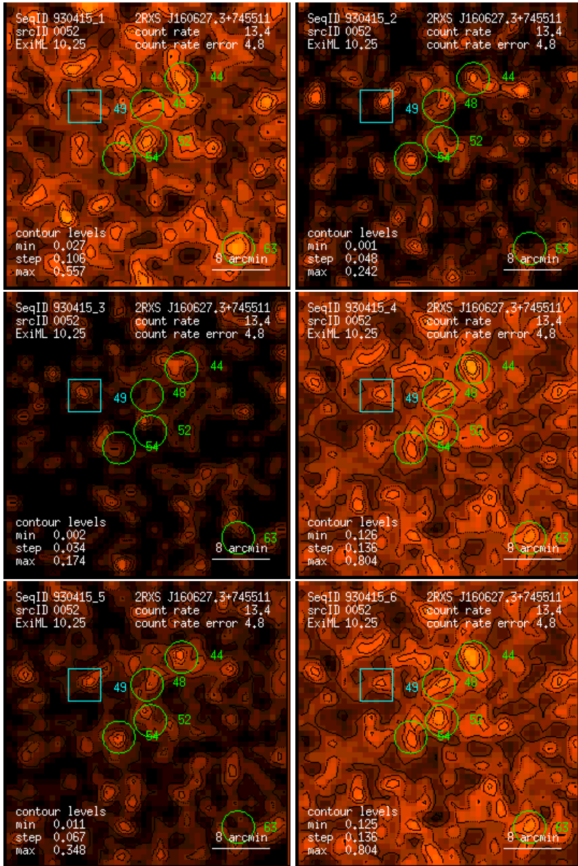
Figure 52: RASS 930415: detection 0052: band rate images, Gaussian filter: (1) PSPC channels 11 – 41, (2) 52 – 90, (3) 91 – 201, (4) 11 – 235, (5) 52 – 201, (6) 11 – 201. Broad band rates in counts/ks. Band rate contour levels in counts/ks/arcmin 2 .
