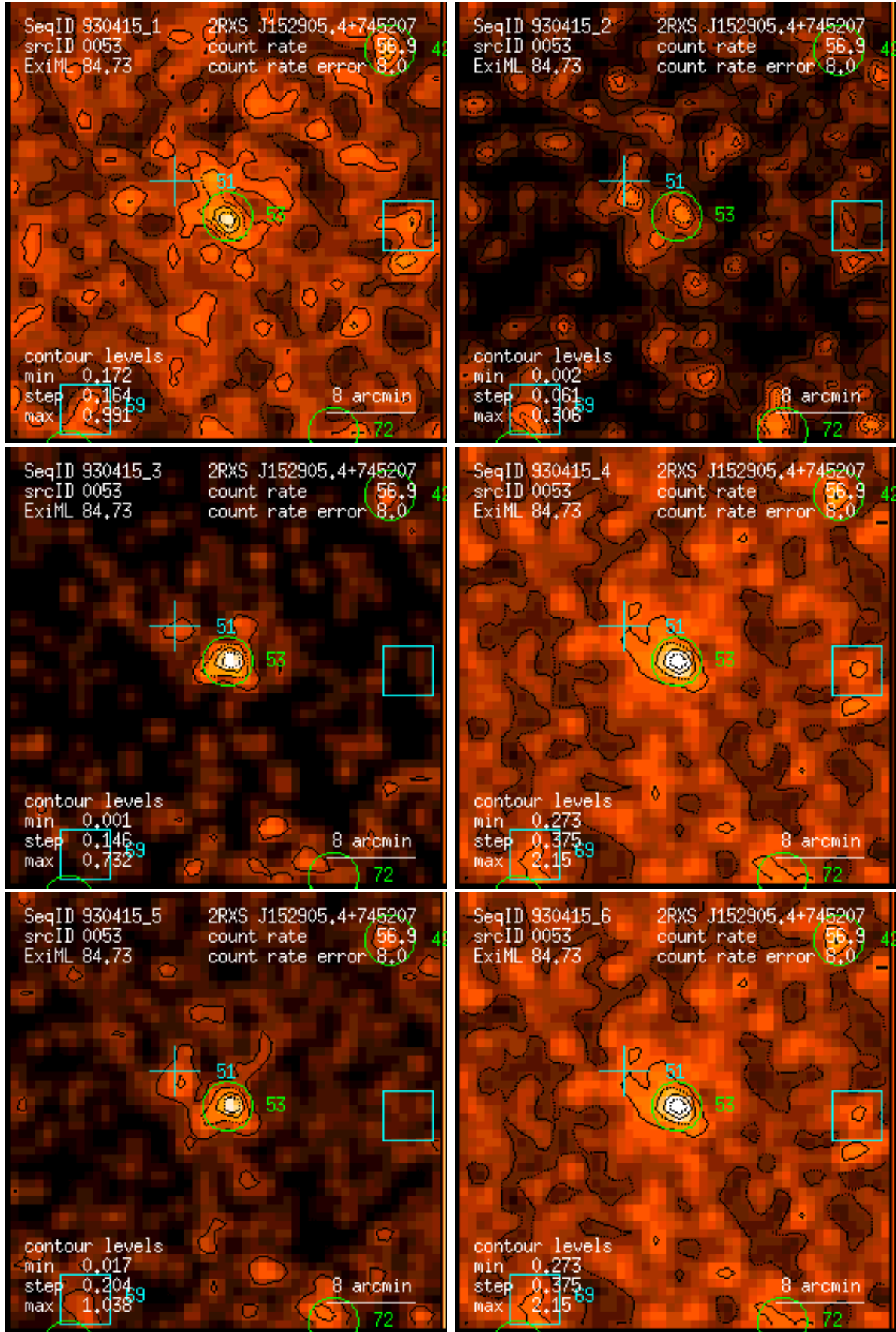
Figure 53: RASS 930415: detection 0053: band rate images, Gaussian filter: (1) PSPC channels 11 – 41, (2) 52 – 90, (3) 91 – 201, (4) 11 – 235, (5) 52 – 201, (6) 11 – 201. Broad band rates in counts/ks. Band rate contour levels in counts/ks/arcmin 2 .
