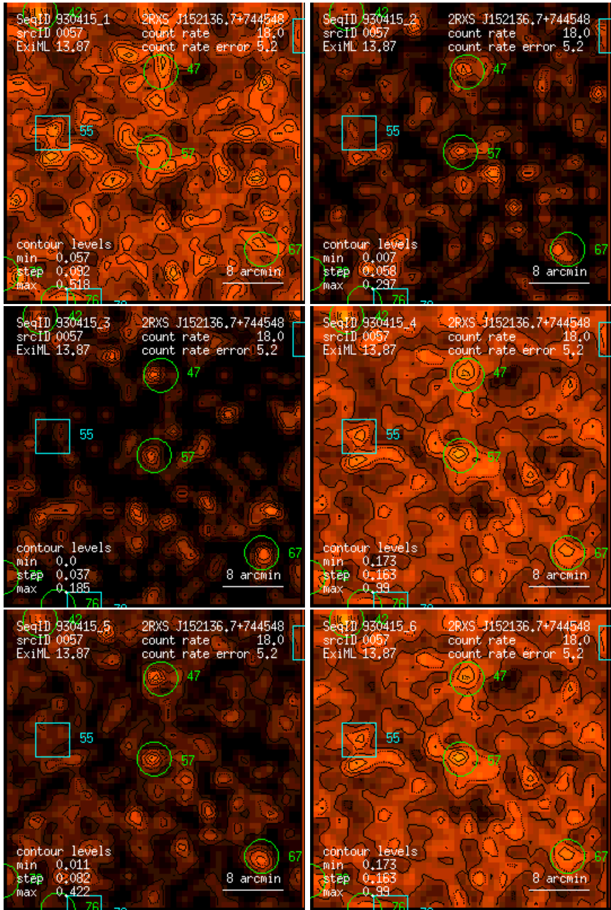
Figure 57: RASS 930415: detection 0057: band rate images, Gaussian filter: (1) PSPC channels 11 – 41, (2) 52 – 90, (3) 91 – 201, (4) 11 – 235, (5) 52 – 201, (6) 11 – 201. Broad band rates in counts/ks. Band rate contour levels in counts/ks/arcmin 2 .
