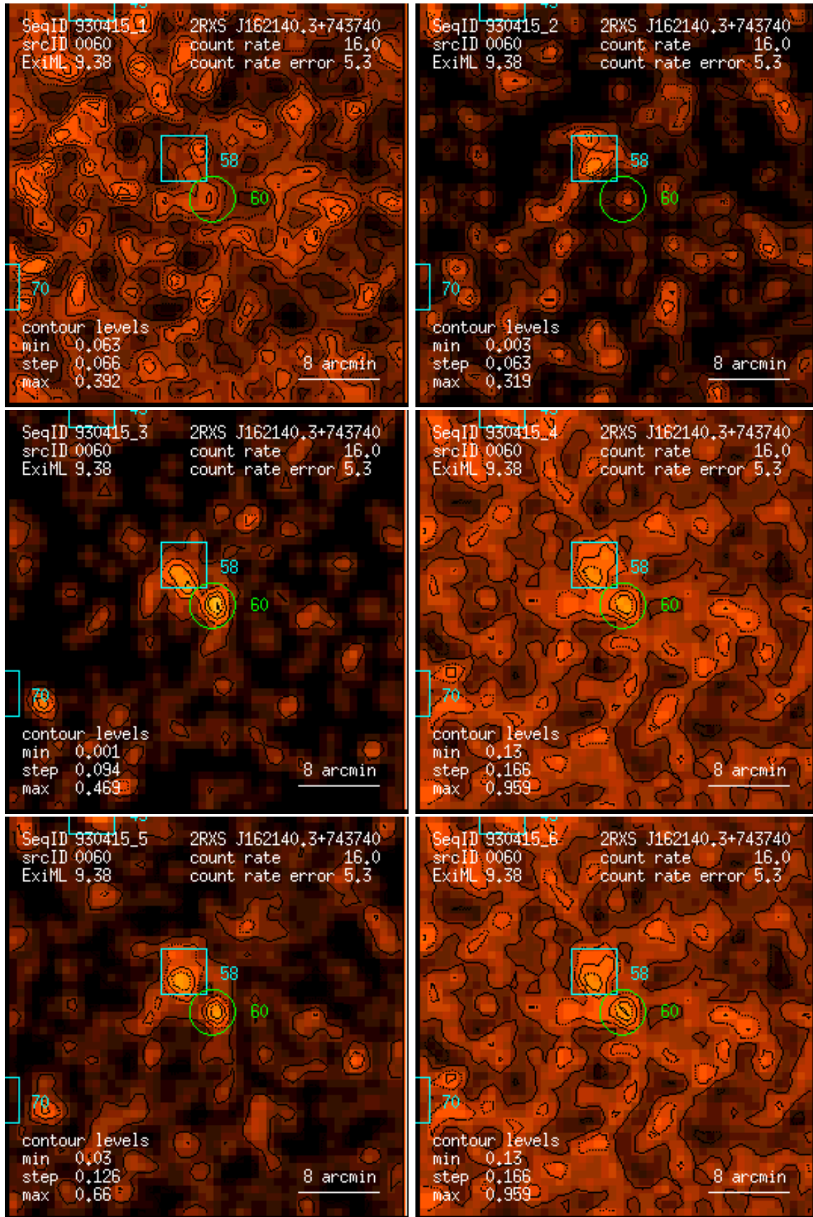
Figure 60: RASS 930415: detection 0060: band rate images, Gaussian filter: (1) PSPC channels 11 – 41, (2) 52 – 90, (3) 91 – 201, (4) 11 – 235, (5) 52 – 201, (6) 11 – 201. Broad band rates in counts/ks. Band rate contour levels in counts/ks/arcmin 2 .
