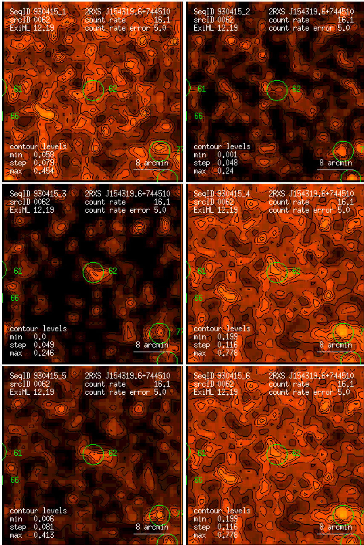
Figure 62: RASS 930415: detection 0062: band rate images, Gaussian filter: (1) PSPC channels 11 – 41, (2) 52 – 90, (3) 91 – 201, (4) 11 – 235, (5) 52 – 201, (6) 11 – 201. Broad band rates in counts/ks. Band rate contour levels in counts/ks/arcmin 2 .
