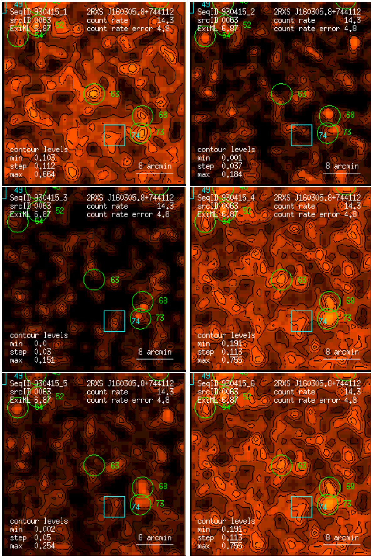
Figure 63: RASS 930415: detection 0063: band rate images, Gaussian filter: (1) PSPC channels 11 – 41, (2) 52 – 90, (3) 91 – 201, (4) 11 – 235, (5) 52 – 201, (6) 11 – 201. Broad band rates in counts/ks. Band rate contour levels in counts/ks/arcmin 2 .
