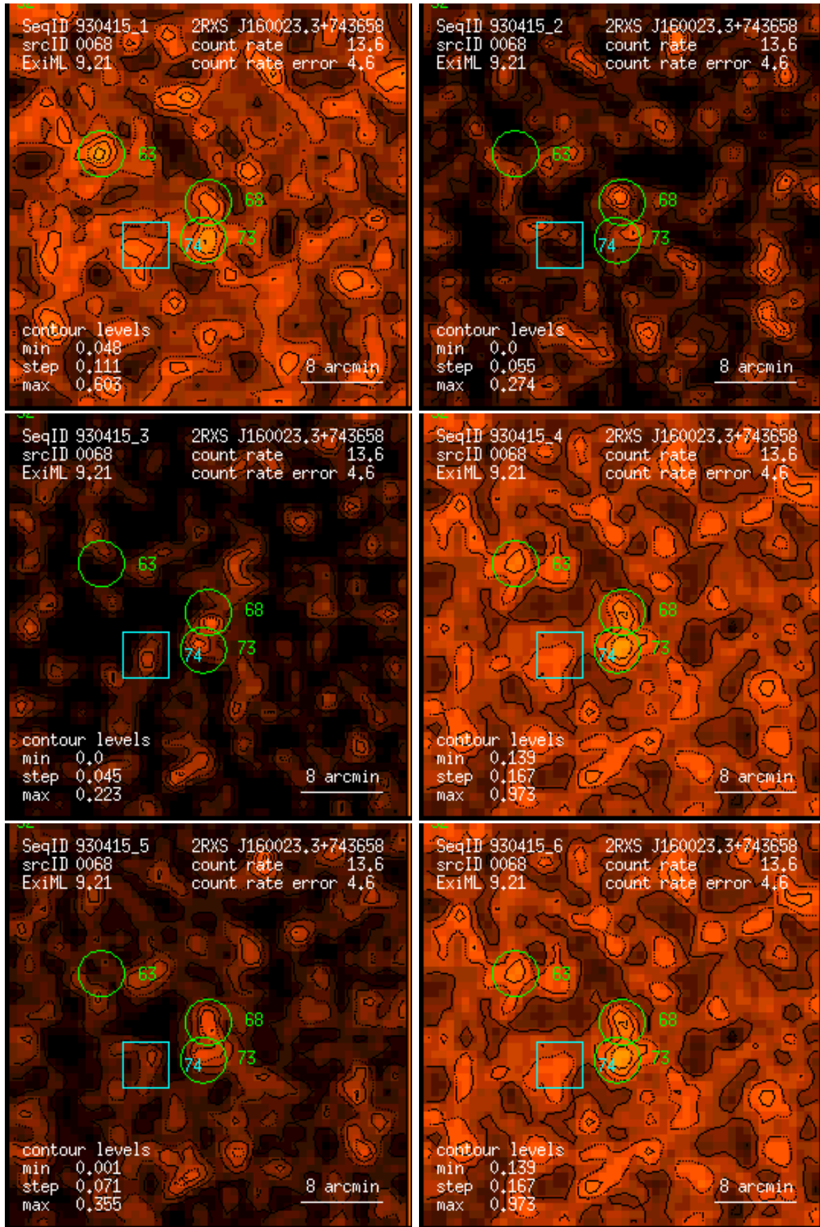
Figure 68: RASS 930415: detection 0068: band rate images, Gaussian filter: (1) PSPC channels 11 – 41, (2) 52 – 90, (3) 91 – 201, (4) 11 – 235, (5) 52 – 201, (6) 11 – 201. Broad band rates in counts/ks. Band rate contour levels in counts/ks/arcmin 2 .
