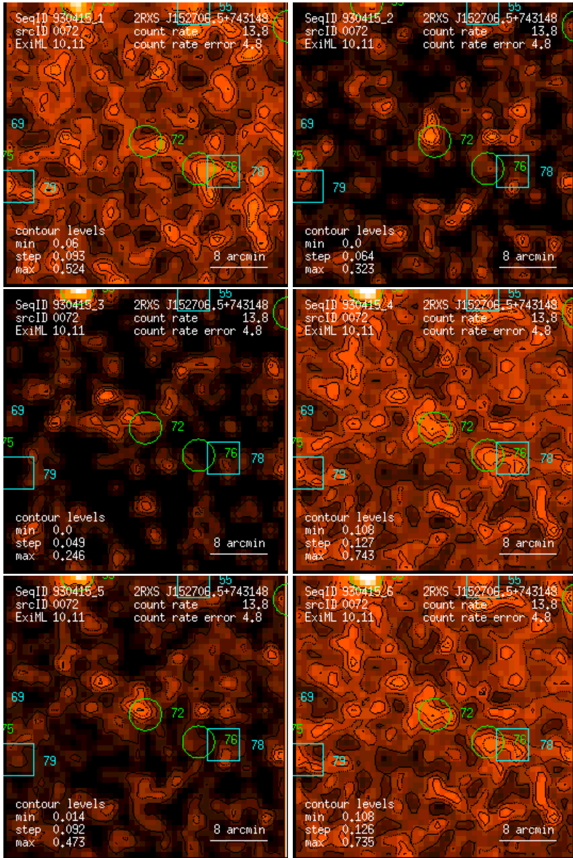
Figure 72: RASS 930415: detection 0072: band rate images, Gaussian filter: (1) PSPC channels 11 – 41, (2) 52 – 90, (3) 91 – 201, (4) 11 – 235, (5) 52 – 201, (6) 11 – 201. Broad band rates in counts/ks. Band rate contour levels in counts/ks/arcmin 2 .
