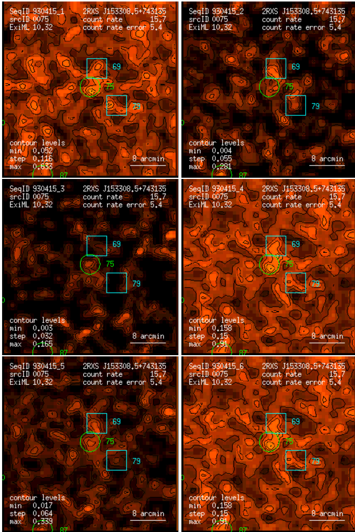
Figure 75: RASS 930415: detection 0075: band rate images, Gaussian filter: (1) PSPC channels 11 – 41, (2) 52 – 90, (3) 91 – 201, (4) 11 – 235, (5) 52 – 201, (6) 11 – 201. Broad band rates in counts/ks. Band rate contour levels in counts/ks/arcmin 2 .
