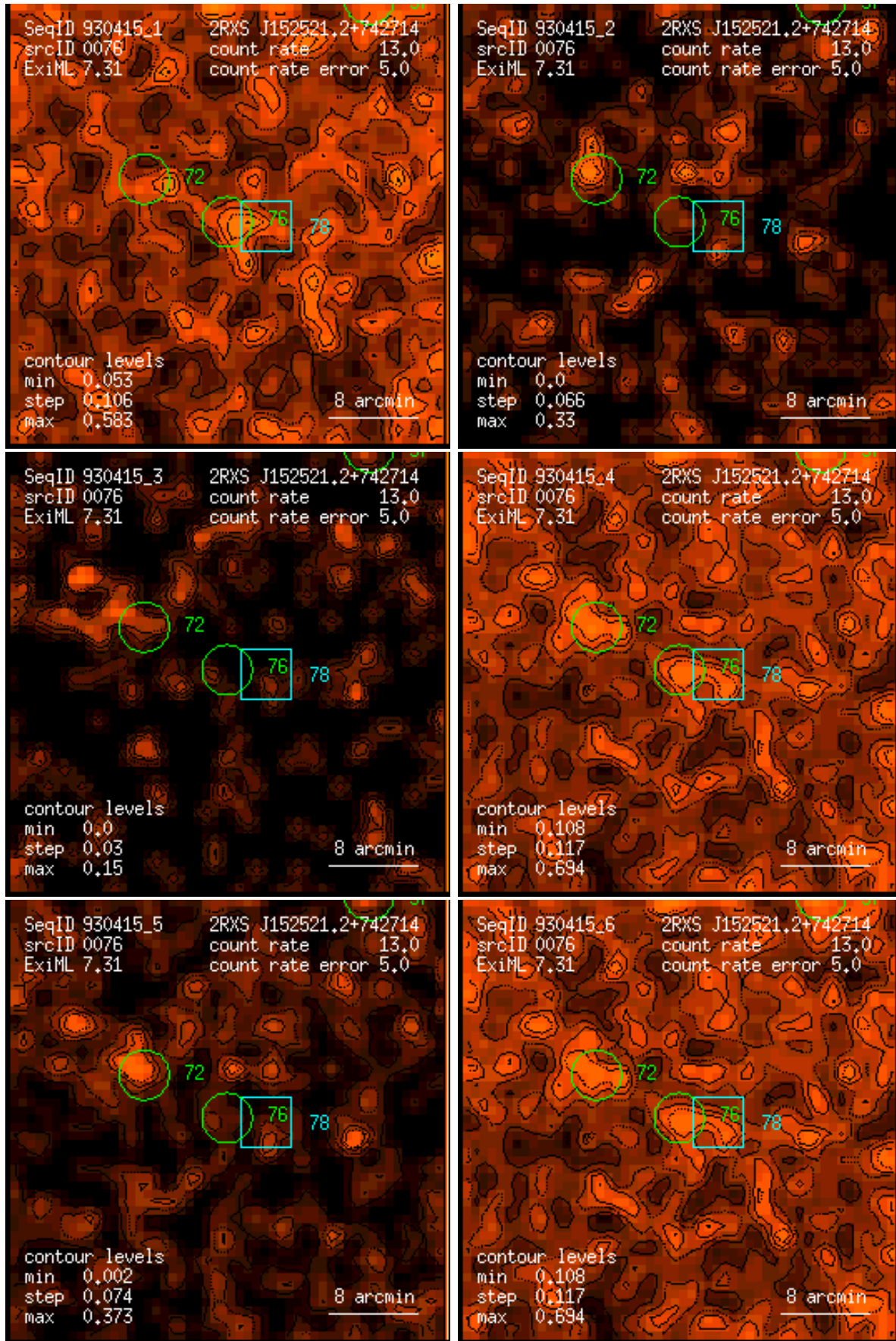
Figure 76: RASS 930415: detection 0076: band rate images, Gaussian filter: (1) PSPC channels 11 – 41, (2) 52 – 90, (3) 91 – 201, (4) 11 – 235, (5) 52 – 201, (6) 11 – 201. Broad band rates in counts/ks. Band rate contour levels in counts/ks/arcmin 2 .
