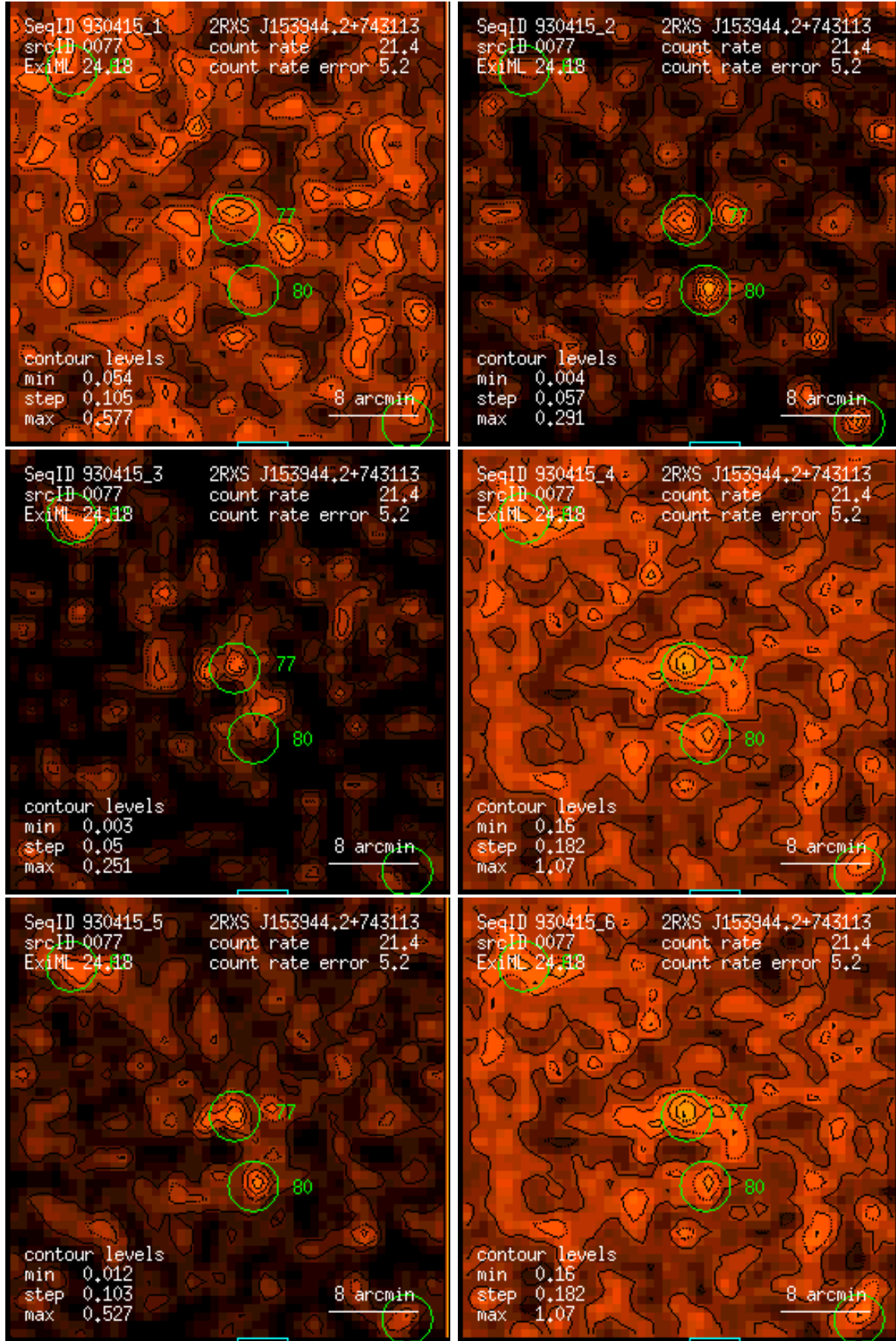
Figure 77: RASS 930415: detection 0077: band rate images, Gaussian filter: (1) PSPC channels 11 – 41, (2) 52 – 90, (3) 91 – 201, (4) 11 – 235, (5) 52 – 201, (6) 11 – 201. Broad band rates in counts/ks. Band rate contour levels in counts/ks/arcmin 2 .
