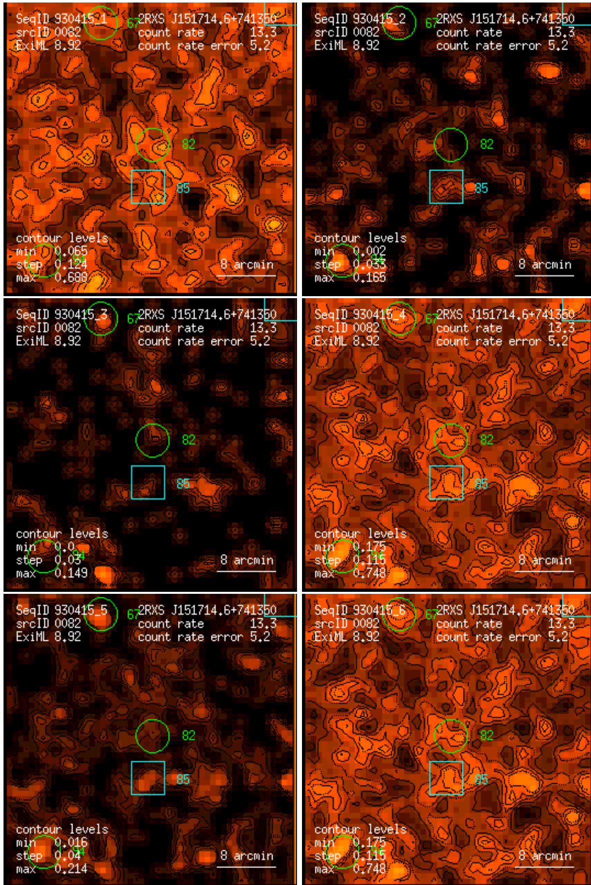
Figure 82: RASS 930415: detection 0082: band rate images, Gaussian filter: (1) PSPC channels 11 – 41, (2) 52 – 90, (3) 91 – 201, (4) 11 – 235, (5) 52 – 201, (6) 11 – 201. Broad band rates in counts/ks. Band rate contour levels in counts/ks/arcmin 2 .
