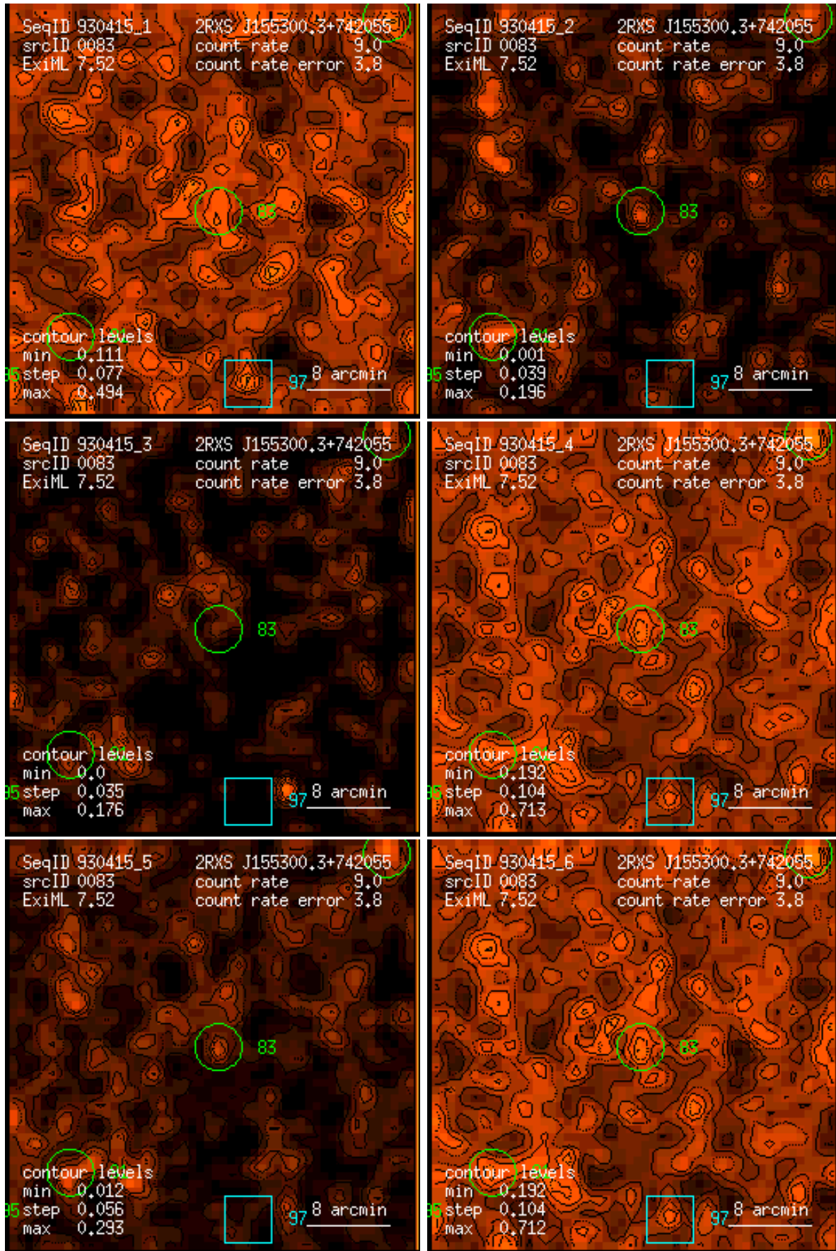
Figure 83: RASS 930415: detection 0083: band rate images, Gaussian filter: (1) PSPC channels 11 – 41, (2) 52 – 90, (3) 91 – 201, (4) 11 – 235, (5) 52 – 201, (6) 11 – 201. Broad band rates in counts/ks. Band rate contour levels in counts/ks/arcmin 2 .
