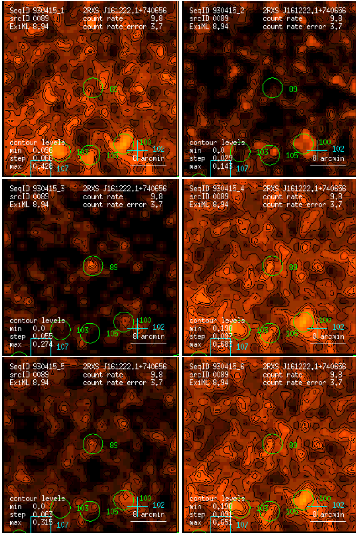
Figure 89: RASS 930415: detection 0089: band rate images, Gaussian filter: (1) PSPC channels 11 – 41, (2) 52 – 90, (3) 91 – 201, (4) 11 – 235, (5) 52 – 201, (6) 11 – 201. Broad band rates in counts/ks. Band rate contour levels in counts/ks/arcmin 2 .
