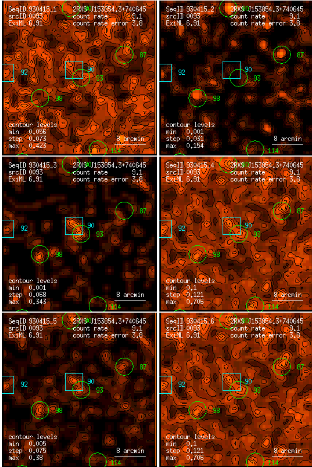
Figure 93: RASS 930415: detection 0093: band rate images, Gaussian filter: (1) PSPC channels 11 – 41, (2) 52 – 90, (3) 91 – 201, (4) 11 – 235, (5) 52 – 201, (6) 11 – 201. Broad band rates in counts/ks. Band rate contour levels in counts/ks/arcmin 2 .
