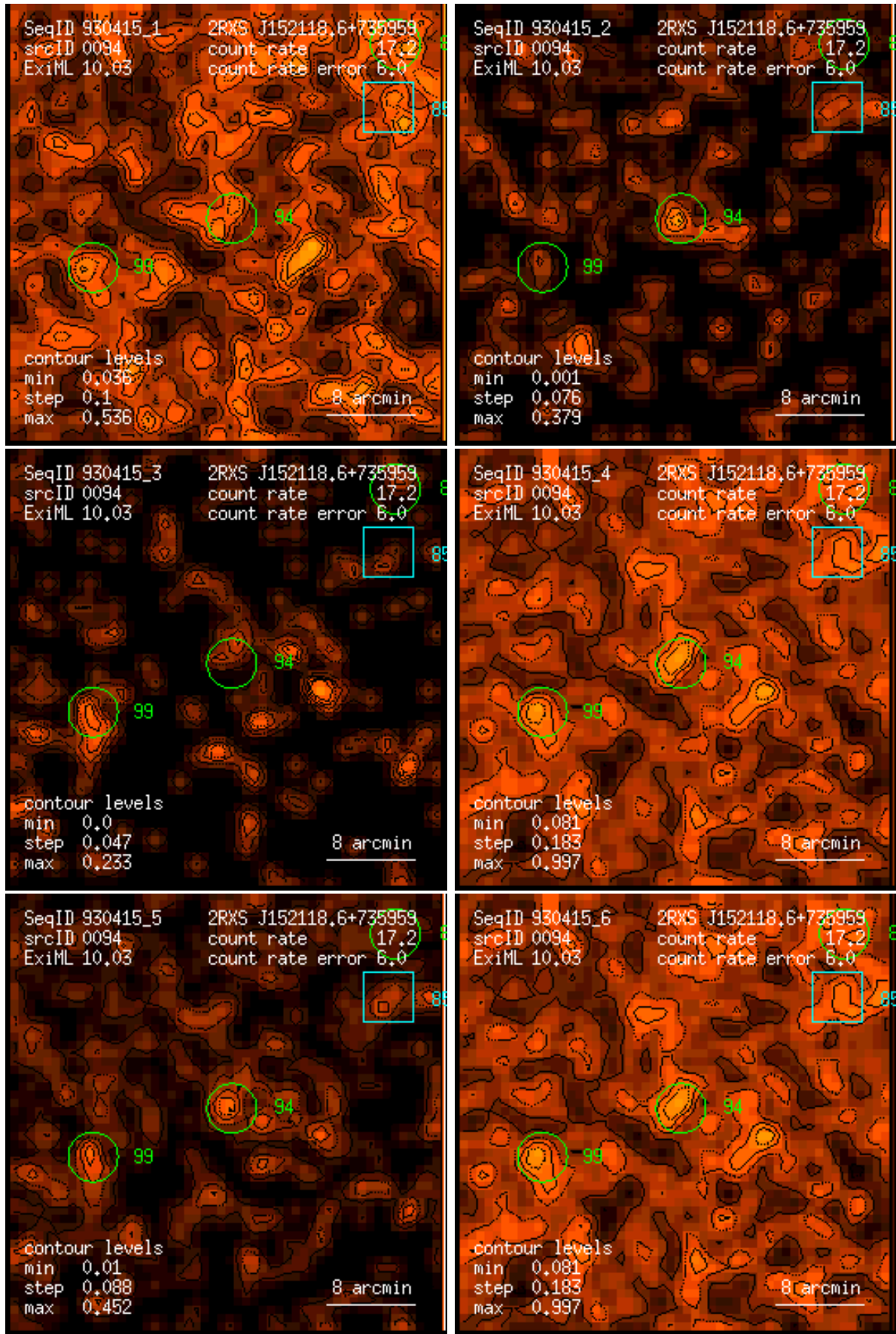
Figure 94: RASS 930415: detection 0094: band rate images, Gaussian filter: (1) PSPC channels 11 – 41, (2) 52 – 90, (3) 91 – 201, (4) 11 – 235, (5) 52 – 201, (6) 11 – 201. Broad band rates in counts/ks. Band rate contour levels in counts/ks/arcmin 2 .
