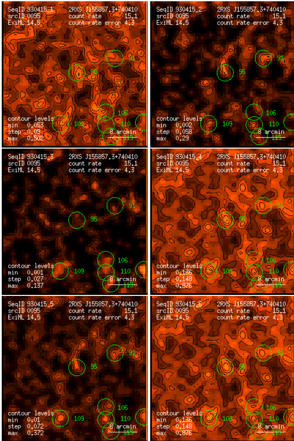
Figure 95: RASS 930415: detection 0095: band rate images, Gaussian filter: (1) PSPC channels 11 – 41, (2) 52 – 90, (3) 91 – 201, (4) 11 – 235, (5) 52 – 201, (6) 11 – 201. Broad band rates in counts/ks. Band rate contour levels in counts/ks/arcmin 2 .
