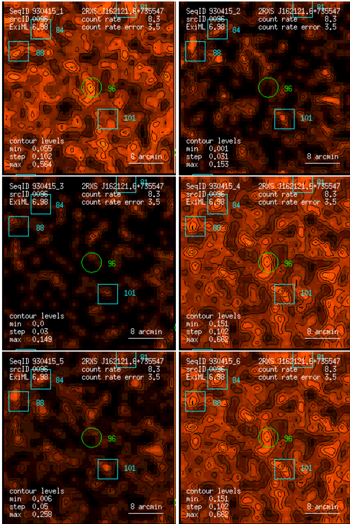
Figure 96: RASS 930415: detection 0096: band rate images, Gaussian filter: (1) PSPC channels 11 – 41, (2) 52 – 90, (3) 91 – 201, (4) 11 – 235, (5) 52 – 201, (6) 11 – 201. Broad band rates in counts/ks. Band rate contour levels in counts/ks/arcmin 2 .
