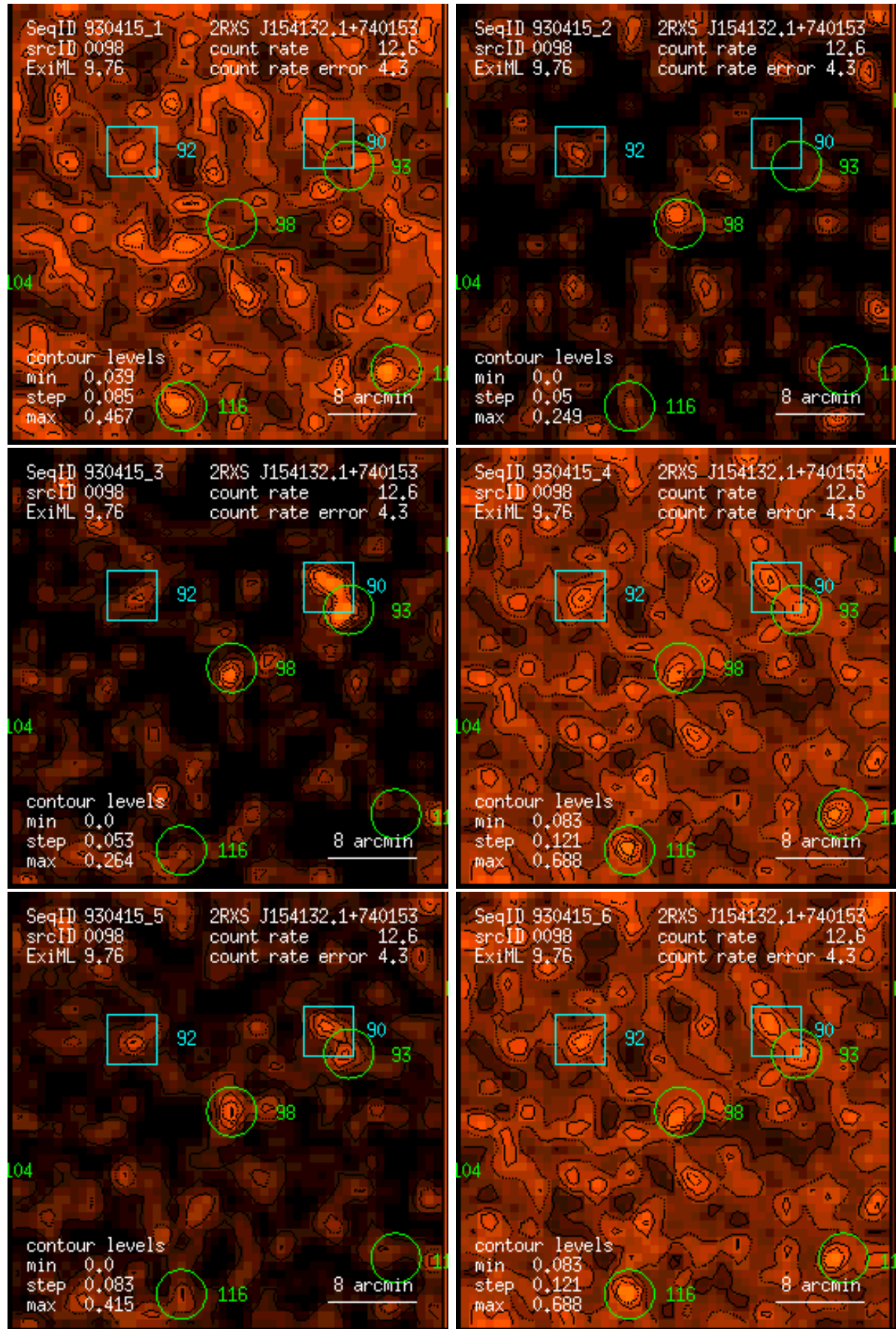
Figure 98: RASS 930415: detection 0098: band rate images, Gaussian filter: (1) PSPC channels 11 – 41, (2) 52 – 90, (3) 91 – 201, (4) 11 – 235, (5) 52 – 201, (6) 11 – 201. Broad band rates in counts/ks. Band rate contour levels in counts/ks/arcmin 2 .
