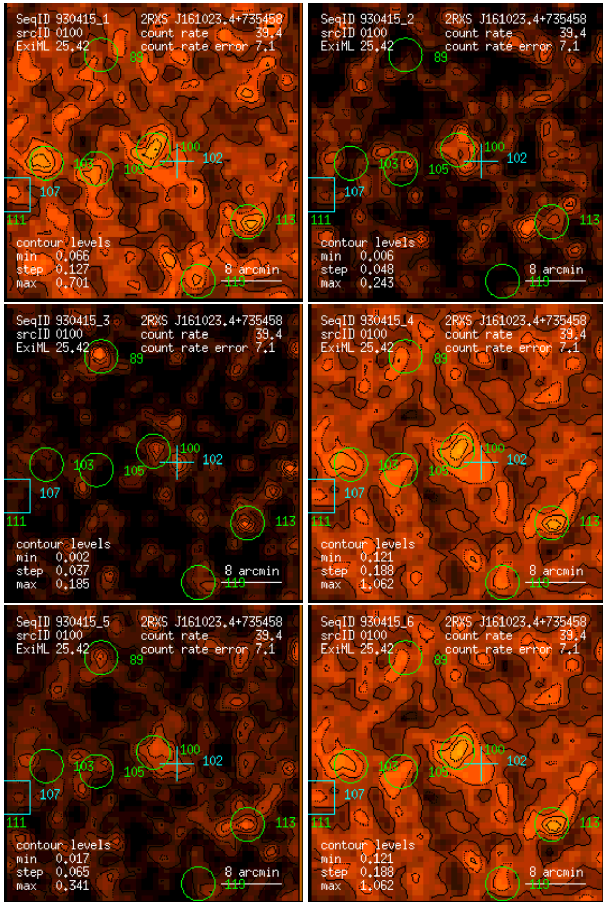
Figure 100: RASS 930415: detection 0100: band rate images, Gaussian filter: (1) PSPC channels 11 – 41, (2) 52 – 90, (3) 91 – 201, (4) 11 – 235, (5) 52 – 201, (6) 11 – 201. Broad band rates in counts/ks. Band rate contour levels in counts/ks/arcmin 2 .
