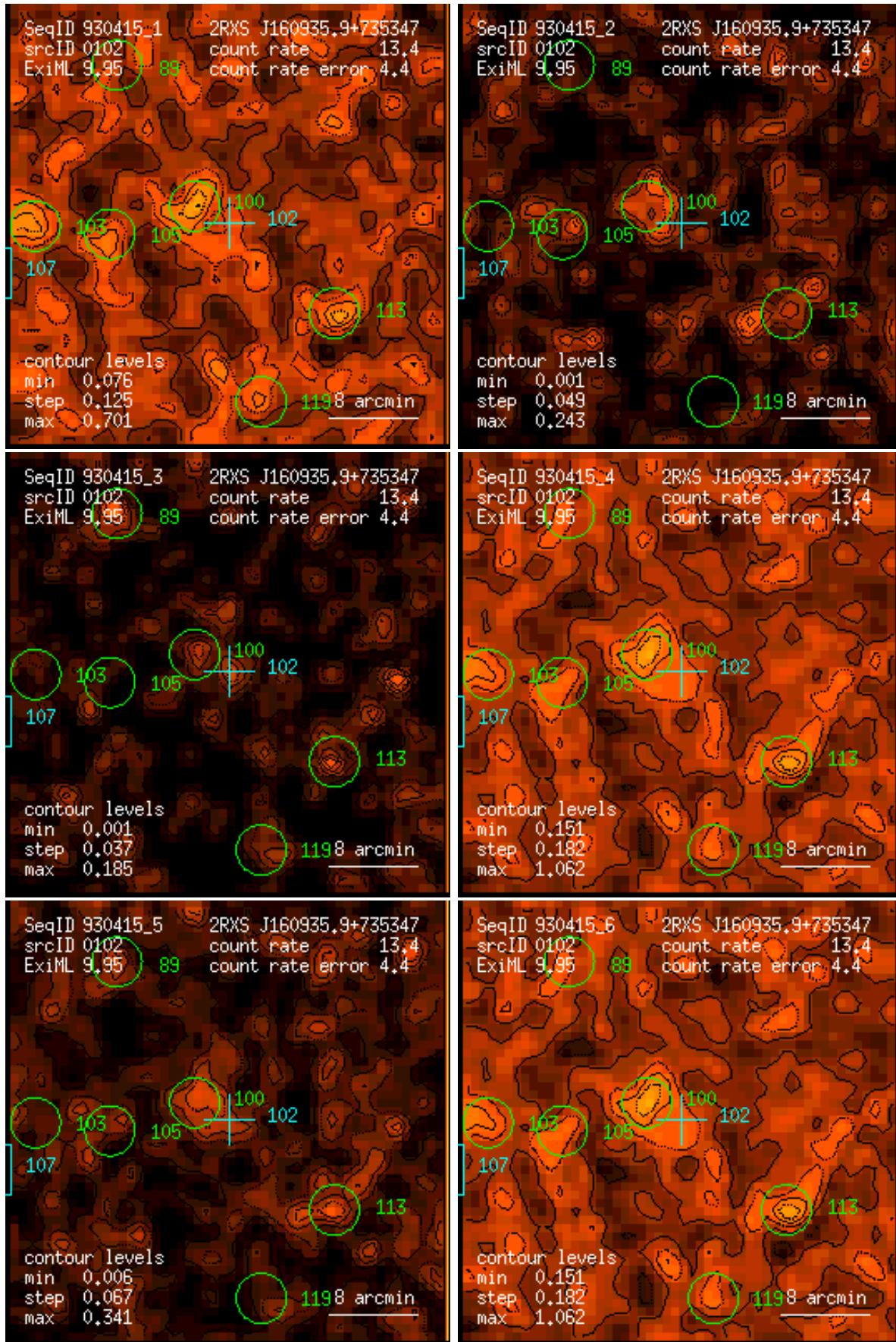
Figure 102: RASS 930415: detection 0102: band rate images, Gaussian filter: (1) PSPC channels 11 – 41, (2) 52 – 90, (3) 91 – 201, (4) 11 – 235, (5) 52 – 201, (6) 11 – 201. Broad band rates in counts/ks. Band rate contour levels in counts/ks/arcmin 2 .
