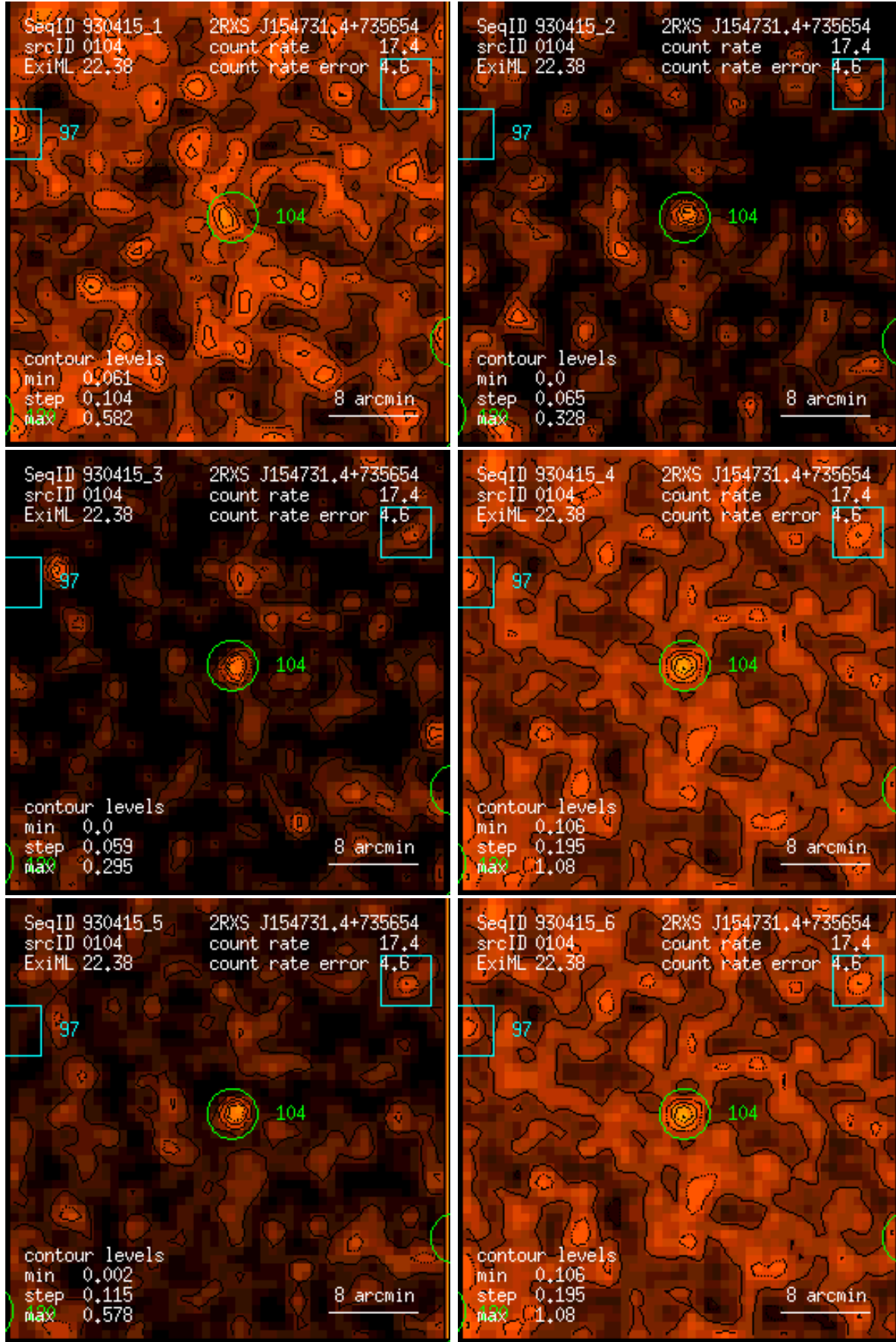
Figure 104: RASS 930415: detection 0104: band rate images, Gaussian filter: (1) PSPC channels 11 – 41, (2) 52 – 90, (3) 91 – 201, (4) 11 – 235, (5) 52 – 201, (6) 11 – 201. Broad band rates in counts/ks. Band rate contour levels in counts/ks/arcmin 2 .
