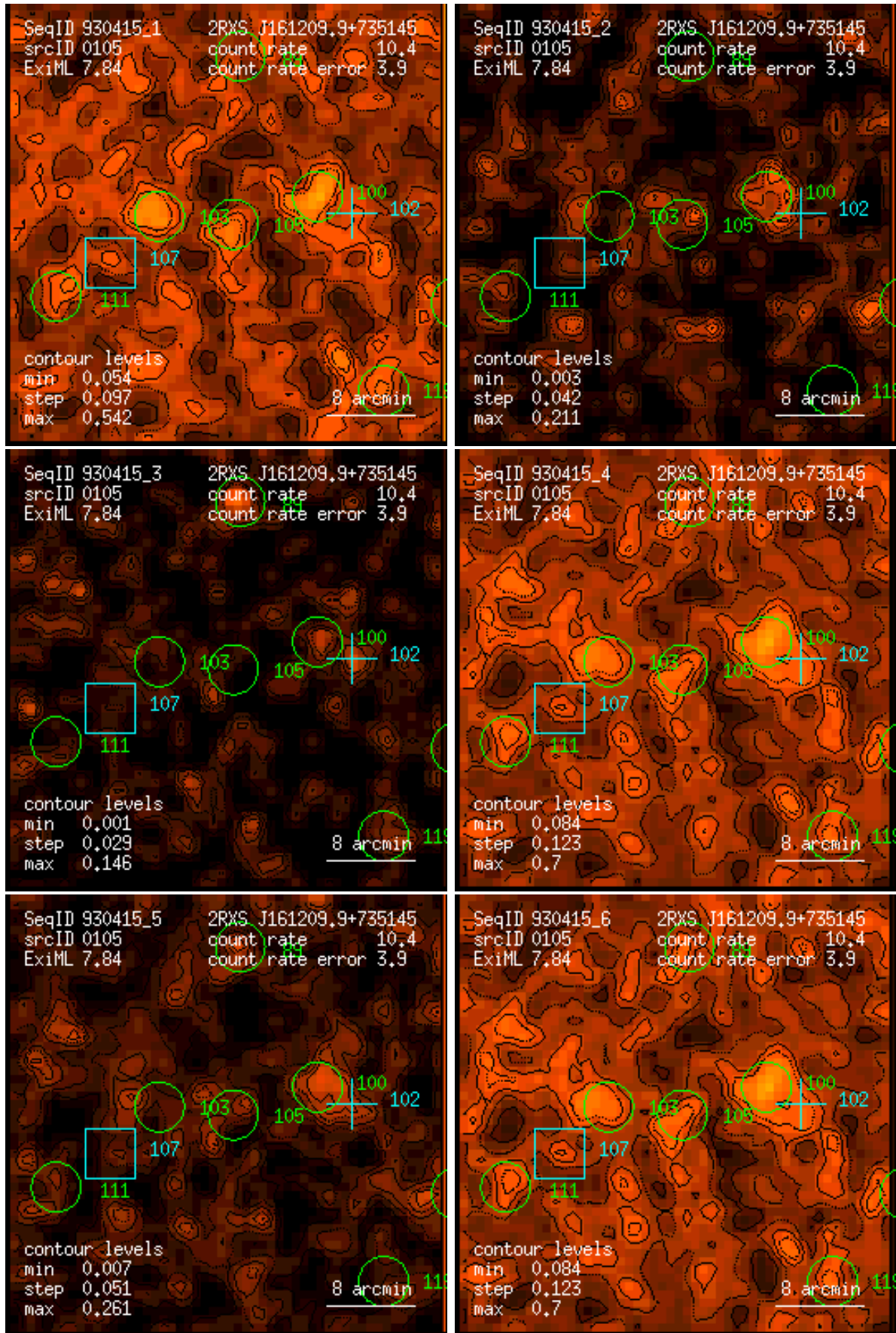
Figure 105: RASS 930415: detection 0105: band rate images, Gaussian filter: (1) PSPC channels 11 – 41, (2) 52 – 90, (3) 91 – 201, (4) 11 – 235, (5) 52 – 201, (6) 11 – 201. Broad band rates in counts/ks. Band rate contour levels in counts/ks/arcmin 2 .
