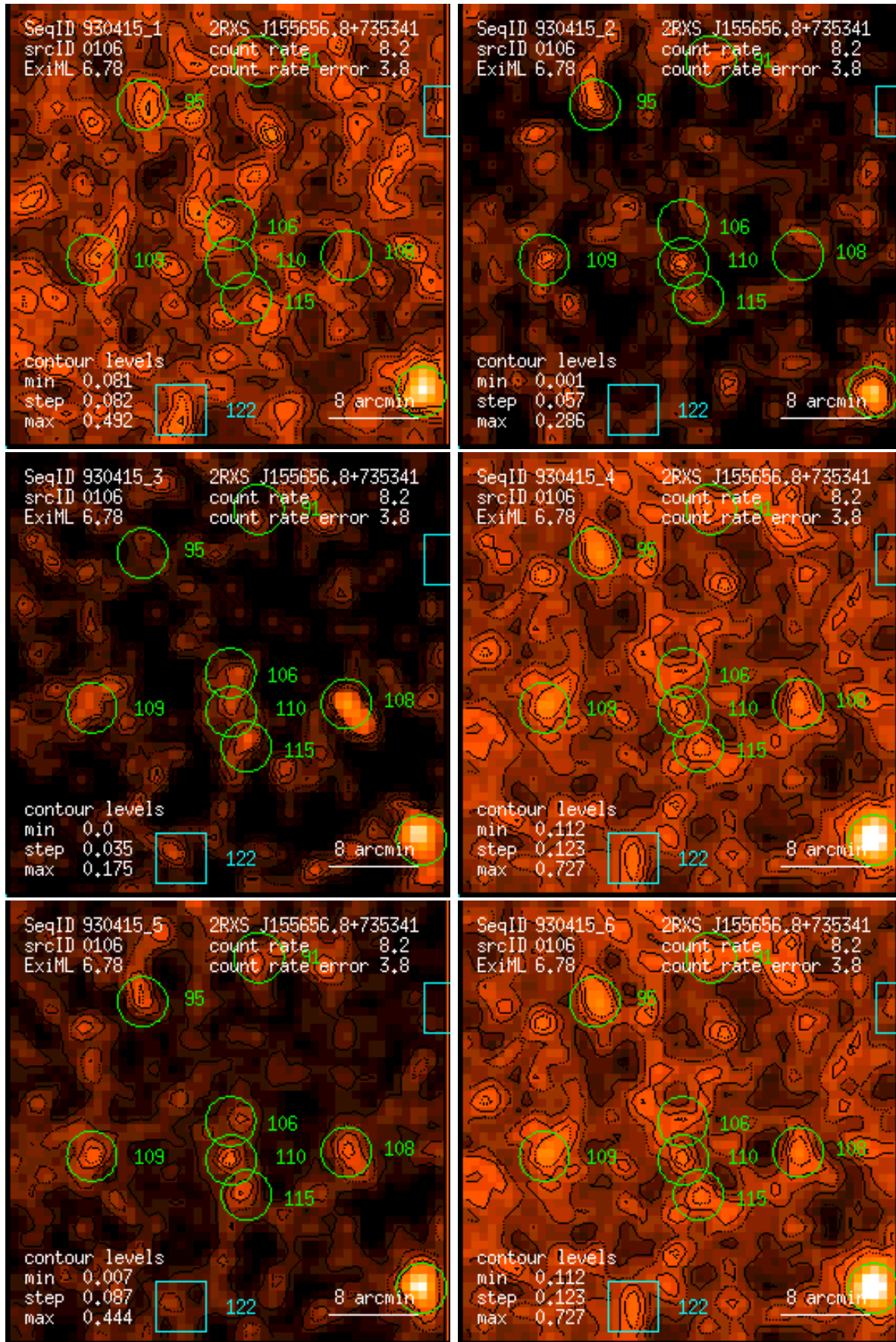
Figure 106: RASS 930415: detection 0106: band rate images, Gaussian filter: (1) PSPC channels 11 – 41, (2) 52 – 90, (3) 91 – 201, (4) 11 – 235, (5) 52 – 201, (6) 11 – 201. Broad band rates in counts/ks. Band rate contour levels in counts/ks/arcmin 2 .
