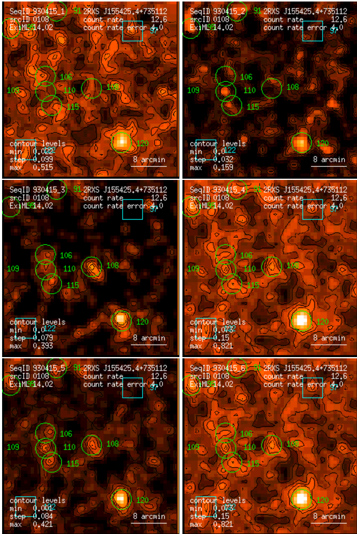
Figure 108: RASS 930415: detection 0108: band rate images, Gaussian filter: (1) PSPC channels 11 – 41, (2) 52 – 90, (3) 91 – 201, (4) 11 – 235, (5) 52 – 201, (6) 11 – 201. Broad band rates in counts/ks. Band rate contour levels in counts/ks/arcmin 2 .
