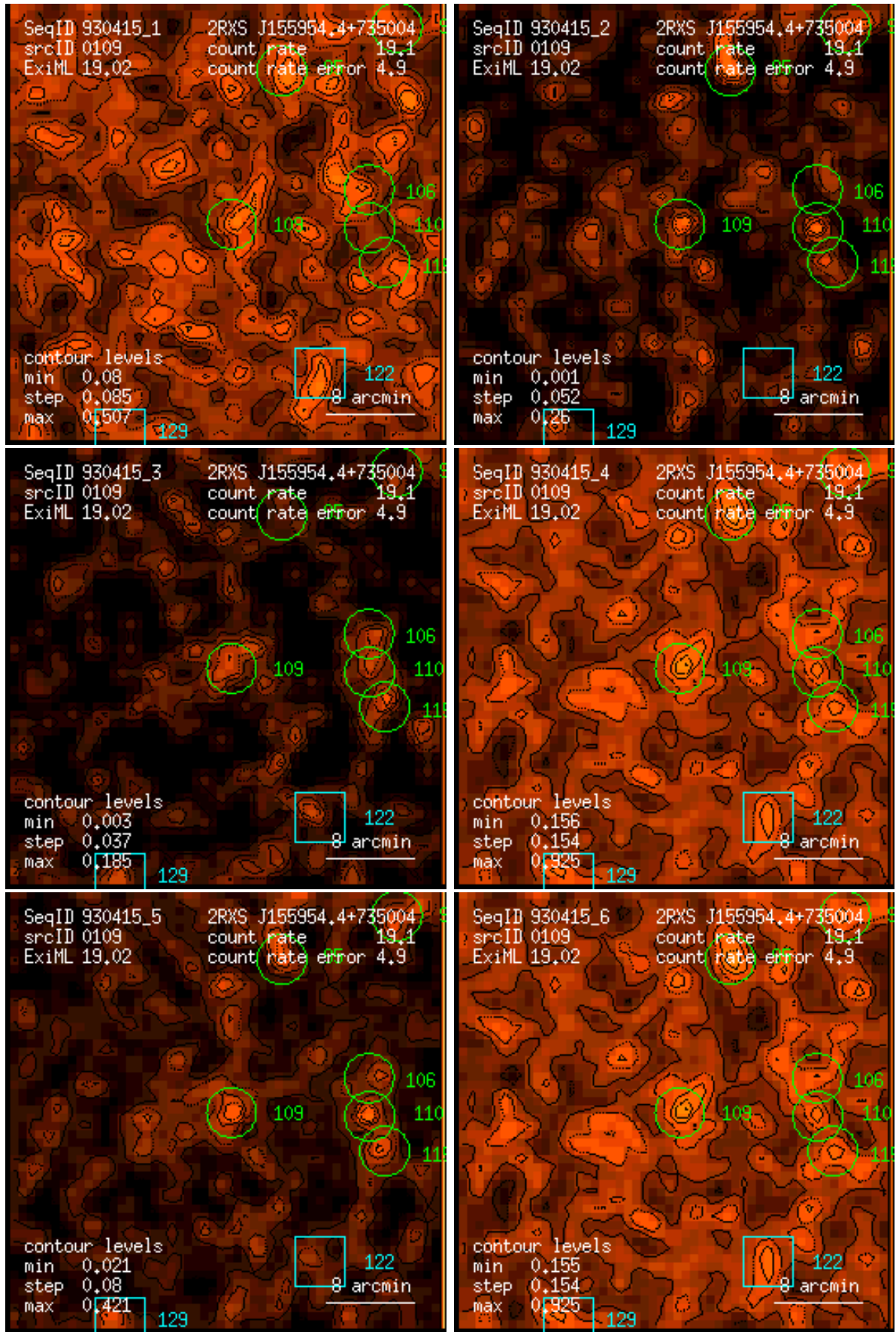
Figure 109: RASS 930415: detection 0109: band rate images, Gaussian filter: (1) PSPC channels 11 – 41, (2) 52 – 90, (3) 91 – 201, (4) 11 – 235, (5) 52 – 201, (6) 11 – 201. Broad band rates in counts/ks. Band rate contour levels in counts/ks/arcmin 2 .
